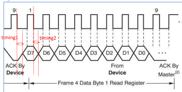
Figure 9. Two-Wire Timing Diagram for Read Word Format
