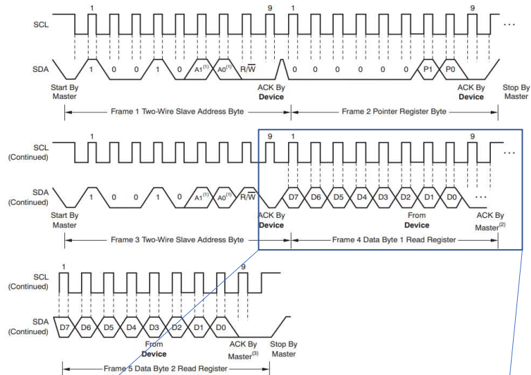
Figure 9. Two-Wire Timing Diagram for Read Word Format
