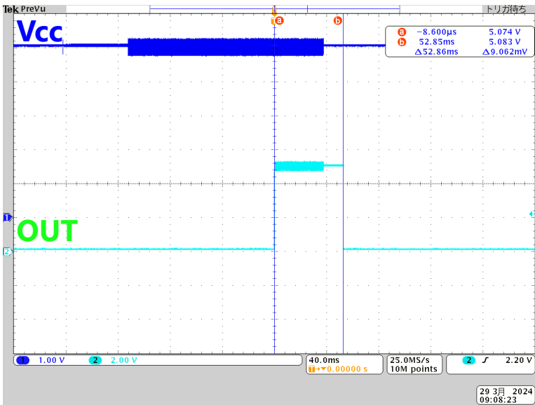
Overall waveform
