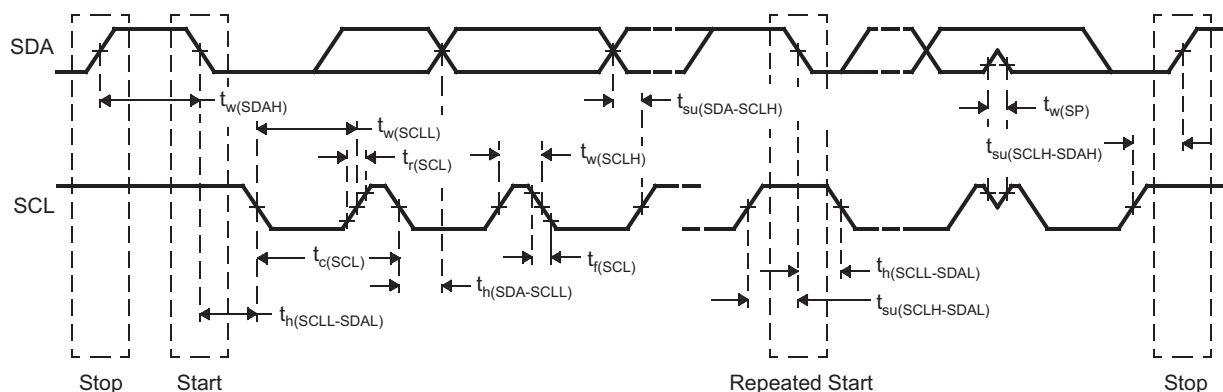
Figure 5-12. I2C Timing Diagram
