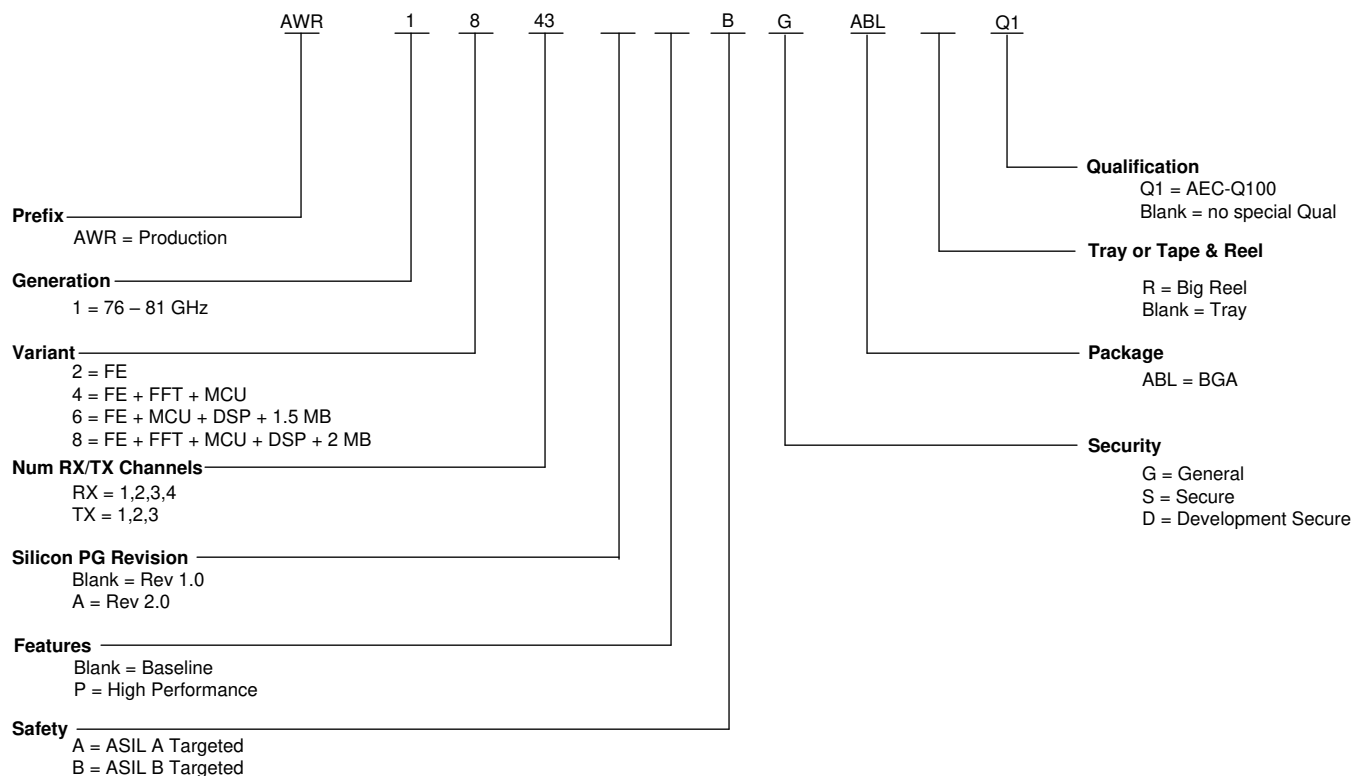
Figure 9-1. Device Nomenclature
