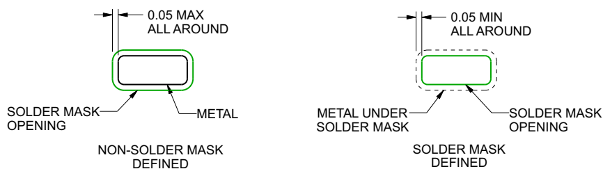
SOLDER MASK DETAIL NOT TO SCALE
