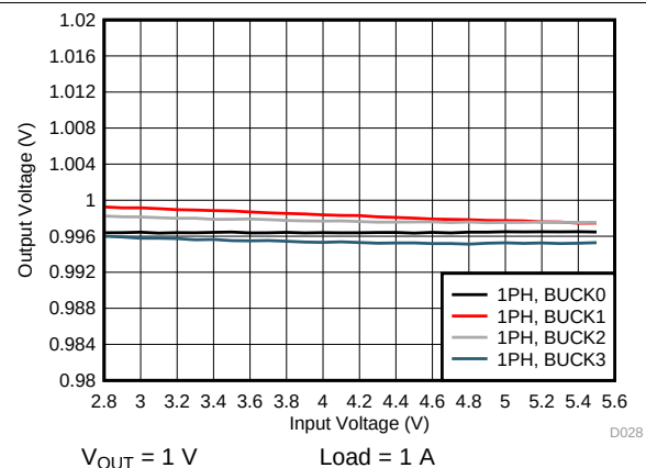
Figure 27. Output Voltage vs Input Voltage in PWM Mode
