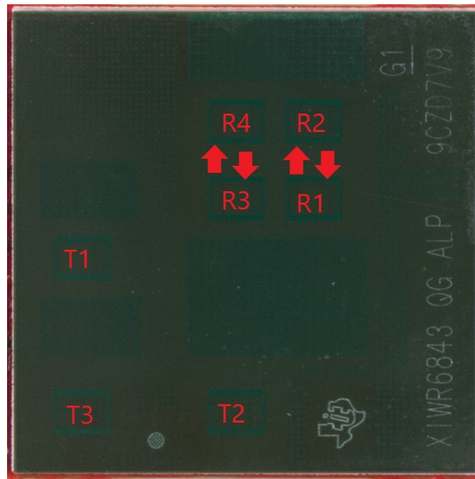
Figure 63. AOP Antennas
