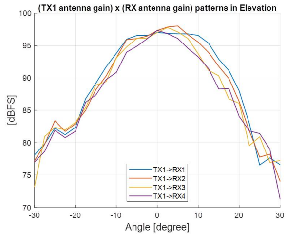
Figure 46. TX1 Antenna Radiation Pattern in Elevation
