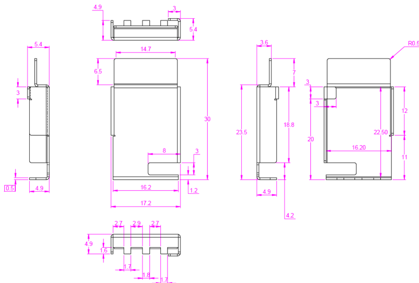
Figure 61. Heat sink CAD drawing
