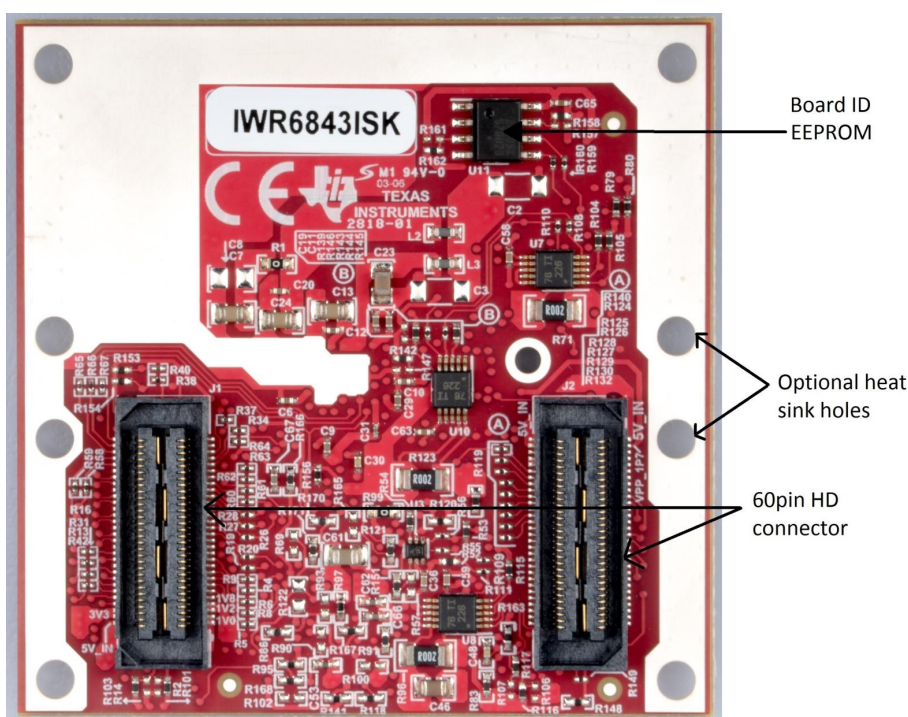
Figure 74. IWR6843ISK Rear View
