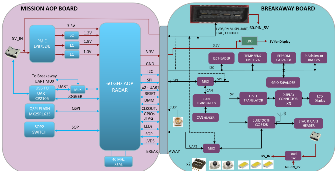
Figure 59. Block Diagram of the IWR6843AOPEVM
