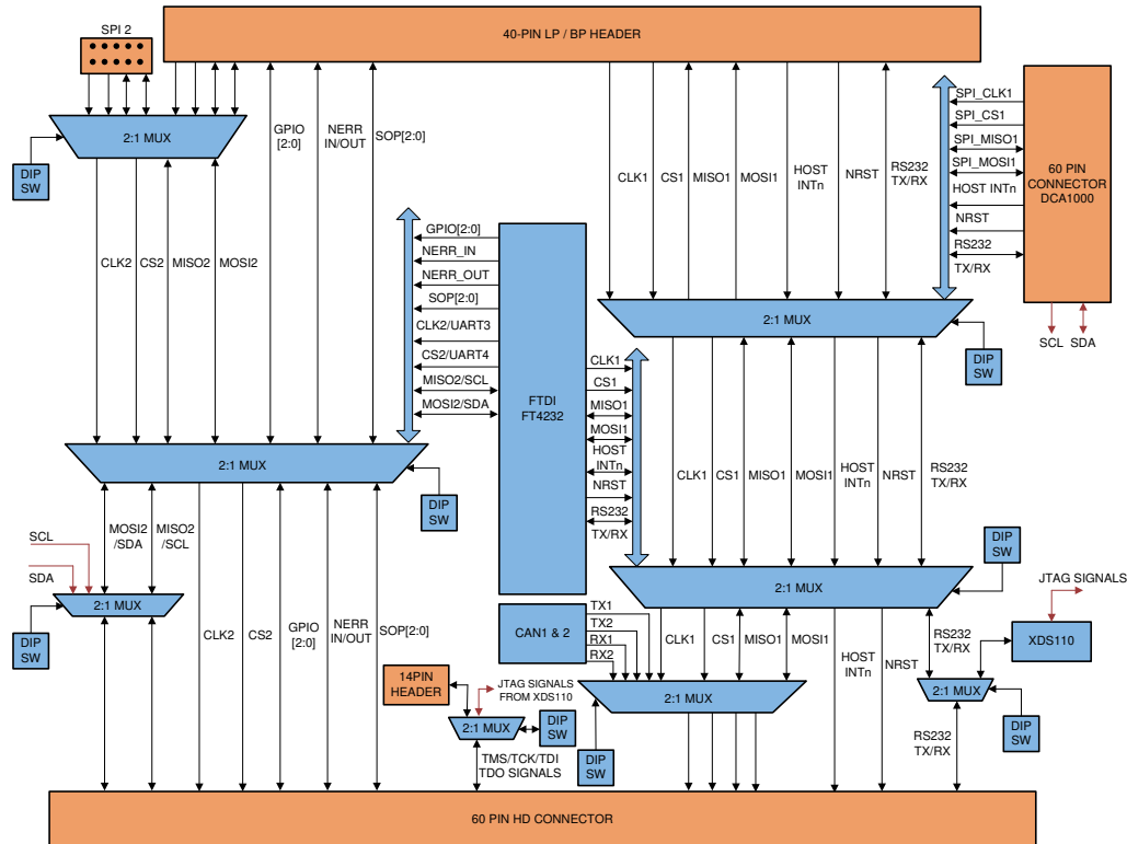
Figure 4. Muxing Scheme
