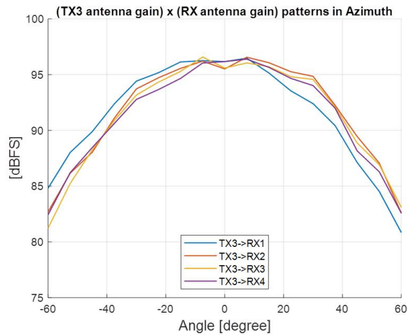
Figure 82. TX3 Antenna Radiation Pattern in Azimuth
