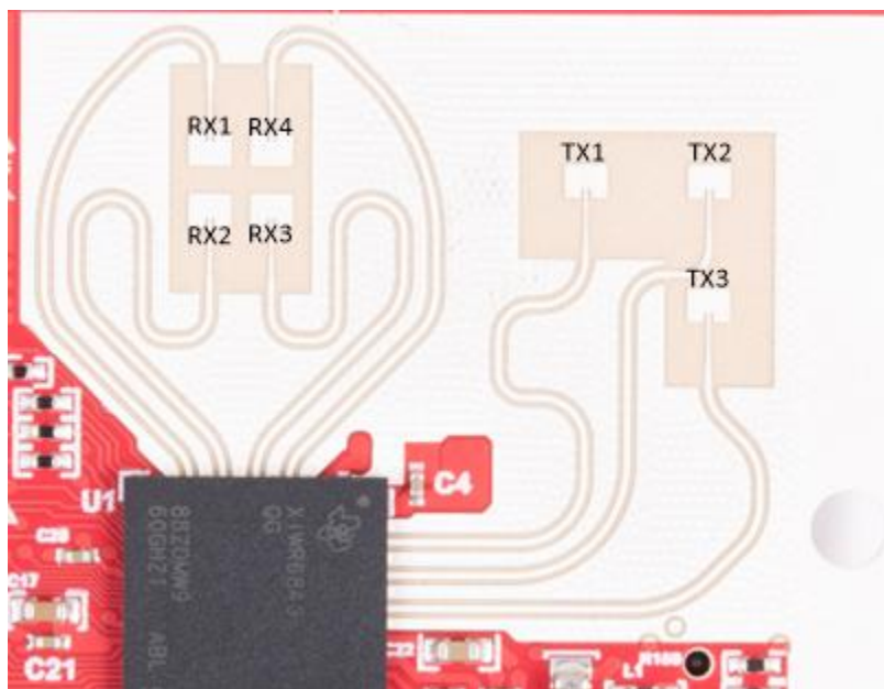
Figure 86. IWR6843ISK-ODS PCB Antenna
