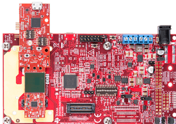
Figure 70. IWR6843AOPEVM Mounted on MMWAVEICBOOST
