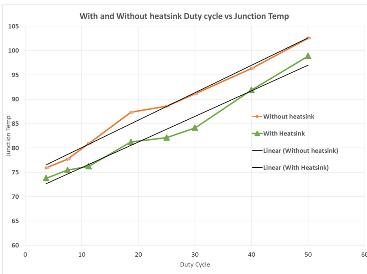
Figure 60. Duty Cycle versus Junction Temperature
