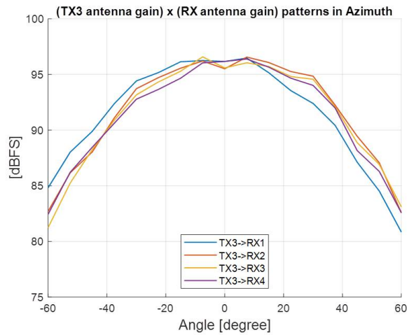
Figure 45. TX3 Antenna Radiation Pattern in Azimuth
