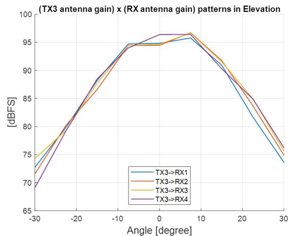
Figure 48. TX3 Antenna Radiation Pattern in Elevation
