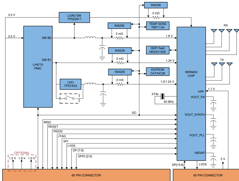
Figure 77. Block Diagram of IWR6843ISK/IWR6843ISK-ODS
