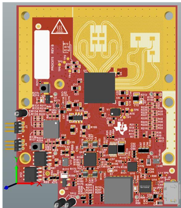
Figure 36. PCB Antenna – Top
