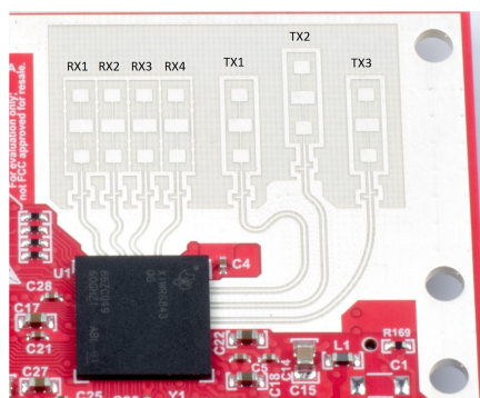
Figure 79. PCB Antennas
