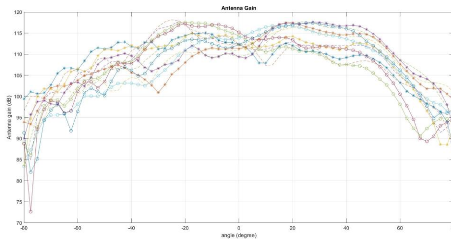
Figure 94. Measured Elevation Radiation Pattern for All Tx to Rx Pairs (All 12 Virtual Antenna Pairs Included)
