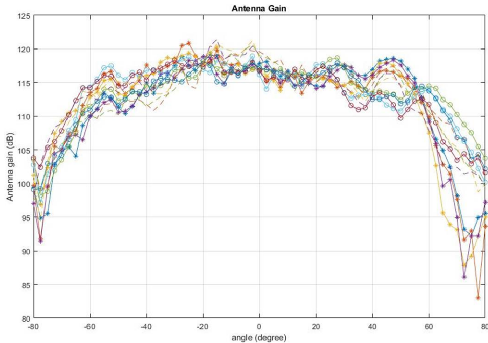
Figure 52. Measured Elevation Radiation Pattern for All Tx to Rx Pairs (All 12 Virtual Antenna Pairs Included)
