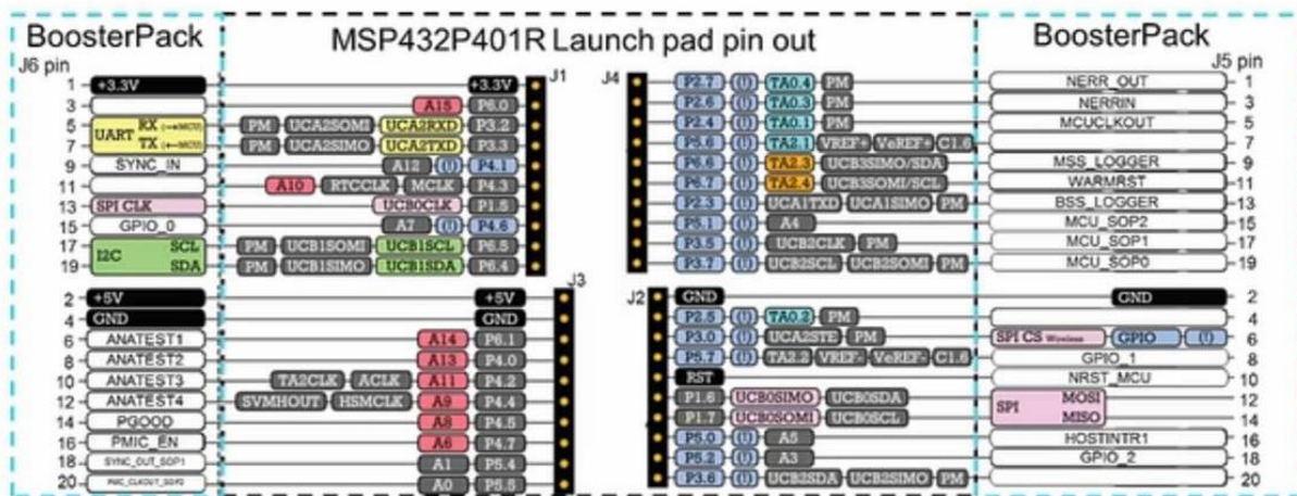
Figure 17. TI Standard LaunchPad
