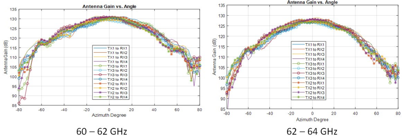
Figure 65. Measured Azimuthal Radiation Pattern for All Tx to Rx Pairs (All 12 Virtual Antenna Pairs Included)
