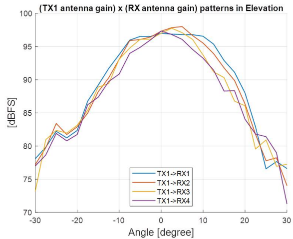
Figure 83. TX1 Antenna Radiation Pattern in Elevation
