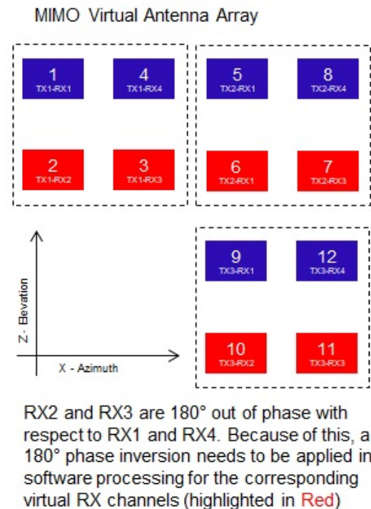
Figure 50. IWR6843ISK-ODS antenna placement MIMO array
