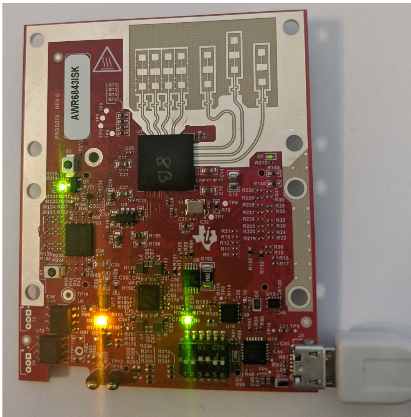
Figure 54. Modular mode setup
