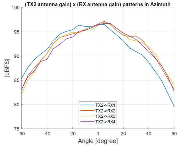
Figure 44. TX2 Antenna Radiation Pattern in Azimuth
