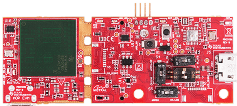
Figure 89. IWR6843AOPEVM Top View
