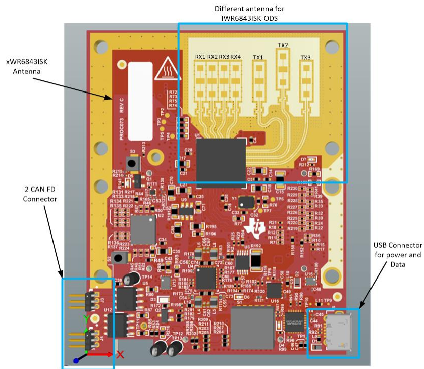
Figure 34. xWR6843ISK Front View
