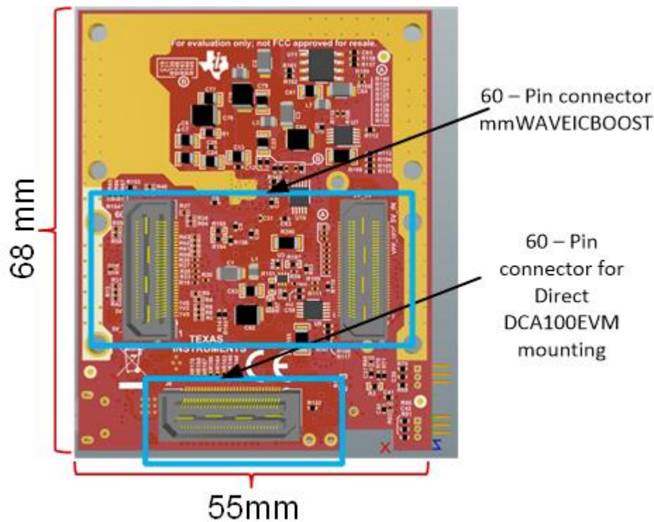
Figure 35. xWR6843ISK Rear View
