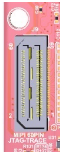
Figure 20. 60-Pin MIPI Connector
