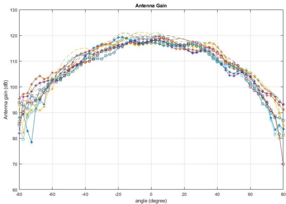
Figure 51. Measured Azimuthal Radiation Pattern for All Tx to Rx Pairs (All 12 Virtual Antenna Pairs Included)
