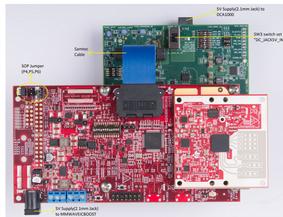
Figure 12. IWR6843ISK-MMWAVEICBOOST-DCA1000EVM Test Setup
