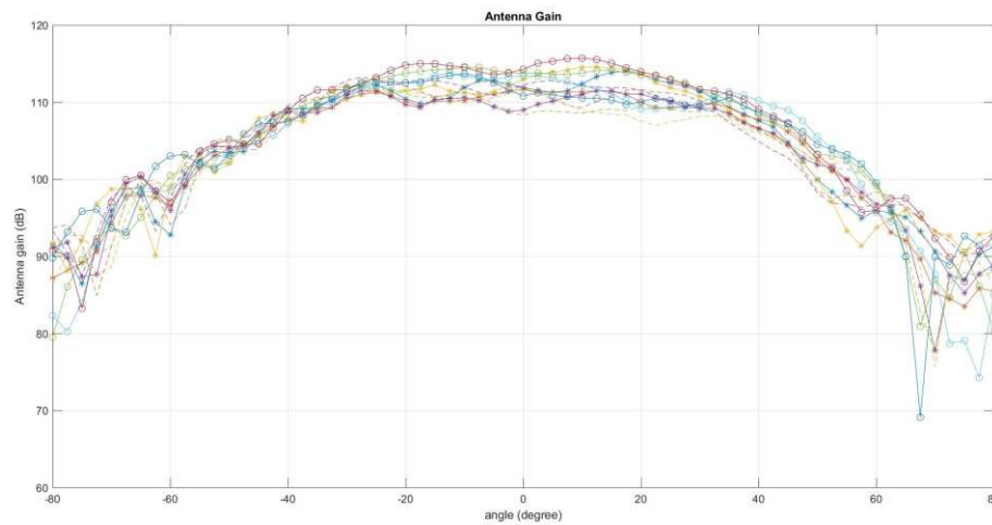
Figure 93. Measured Azimuthal Radiation Pattern for All Tx to Rx Pairs (All 12 Virtual Antenna Pairs Included)
