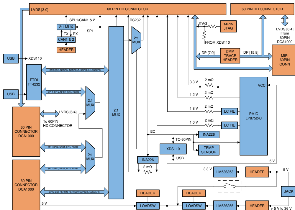
Figure 3. Block Diagram of MMWAVEICBOOST
