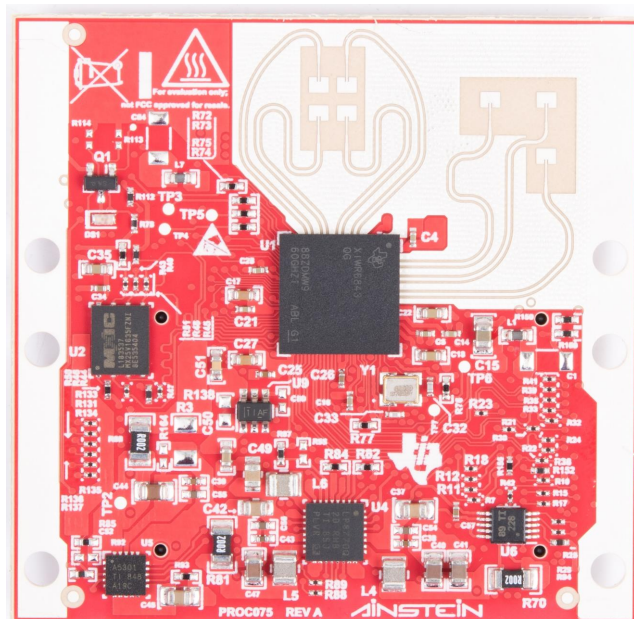
Figure 75. PCB Antenna – Top
