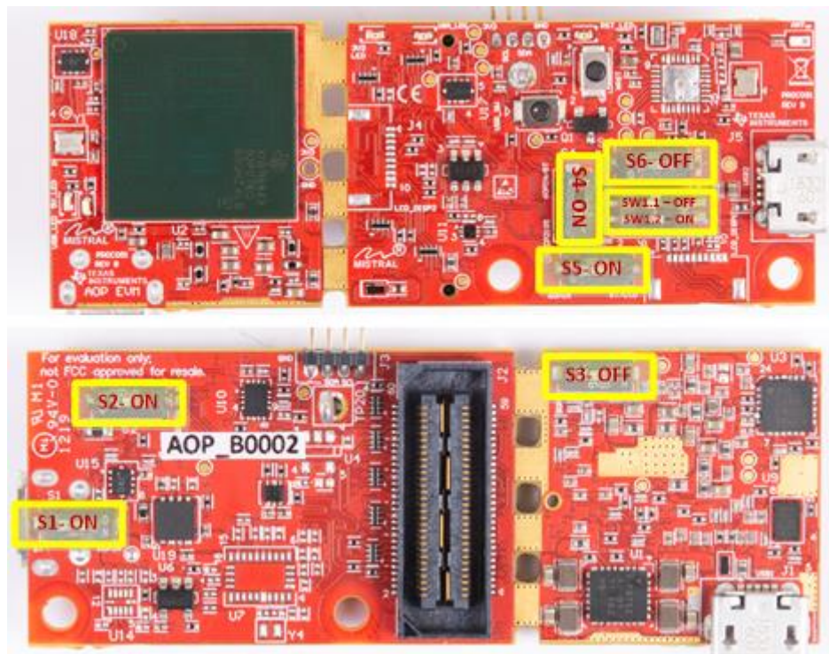
Figure 98. Switch Configuration for MMWAVEICBOOST Mode
