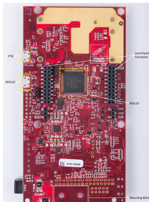
Figure 2. MMWAVEICBOOST Rear View
