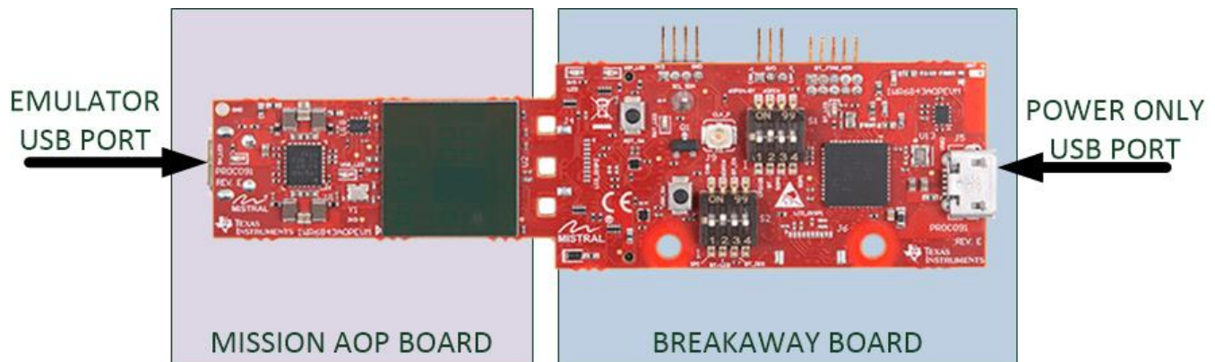
Figure 57. IWR6843AOPEVM Top View
