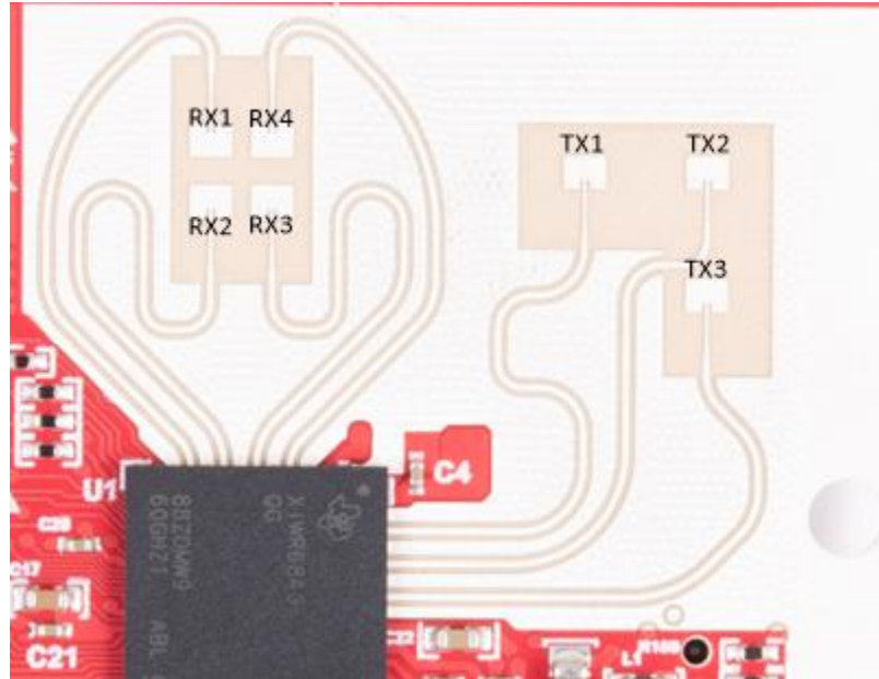
Figure 49. IWR6843ISK-ODS PCB Antenna
