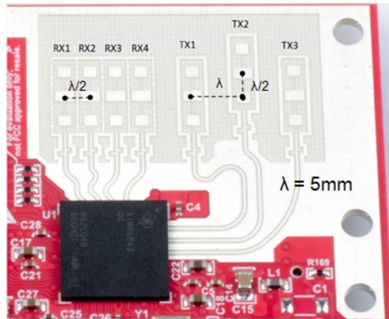
Figure 42. IWR6843ISK antenna placement MIMO array
