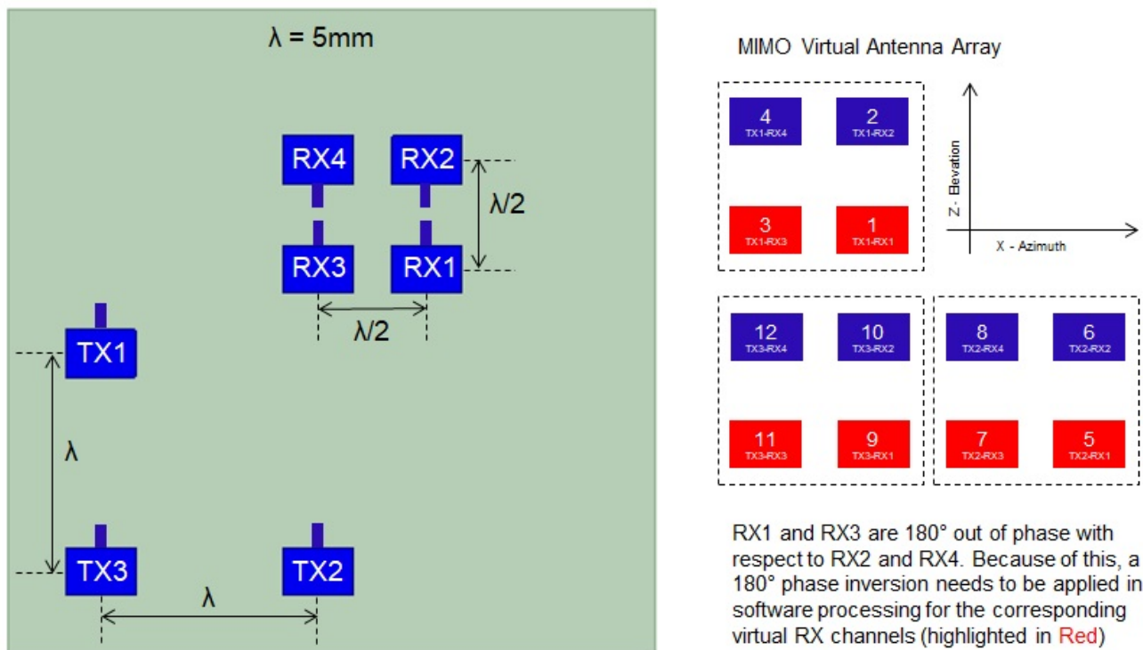
Figure 64. IWR6843AOP antenna placement MIMO array
