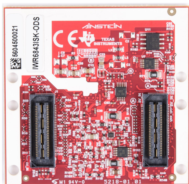
Figure 76. PCB Antenna – Bottom
