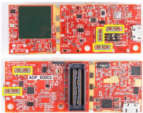
Figure 96. Switch Configuration for Modular Mode
