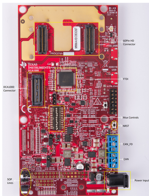
Figure 1. MMWAVEICBOOST Front View
