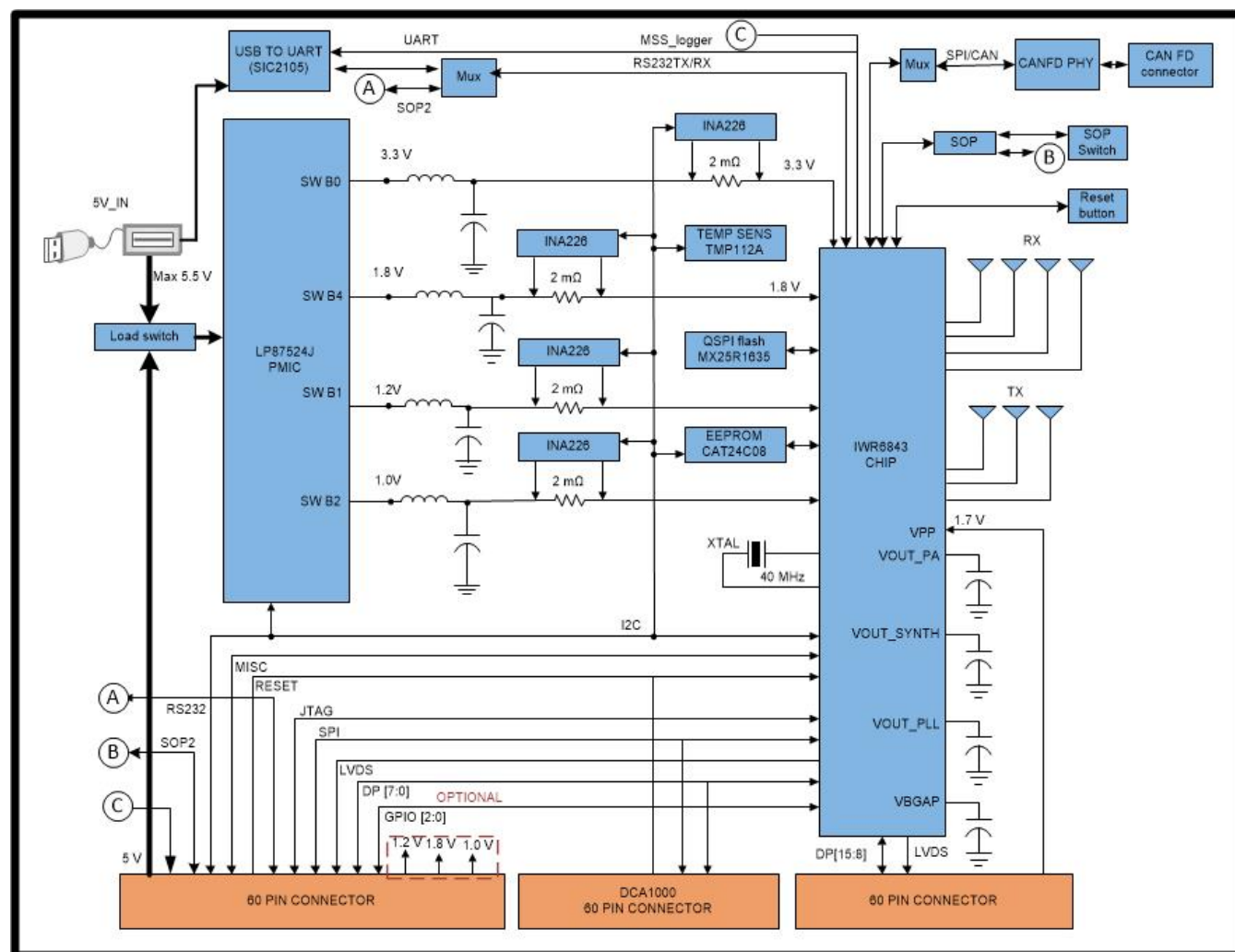
Figure 38. Block Diagram of xWR6843ISK/IWR6843ISK-ODS
