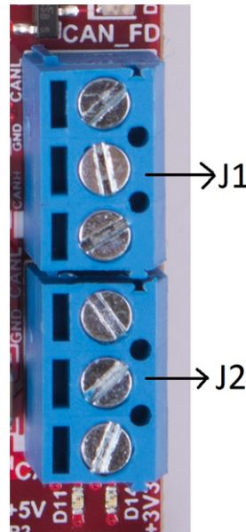
Figure 22. CAN Connectors
