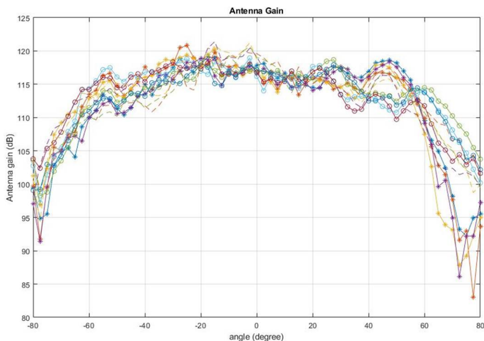
Figure 88. Measured Elevation Radiation Pattern for All Tx to Rx Pairs (All 12 Virtual Antenna Pairs Included)
