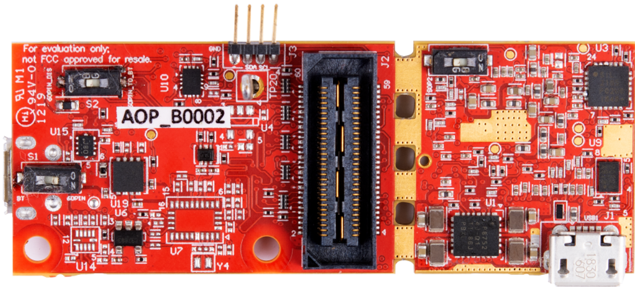
Figure 90. IWR6843AOPEVM Bottom View
