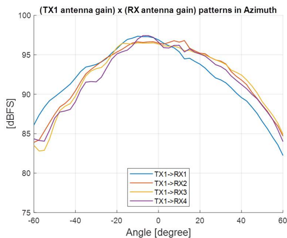
Figure 80. TX1 Antenna Radiation Pattern in Azimuth
