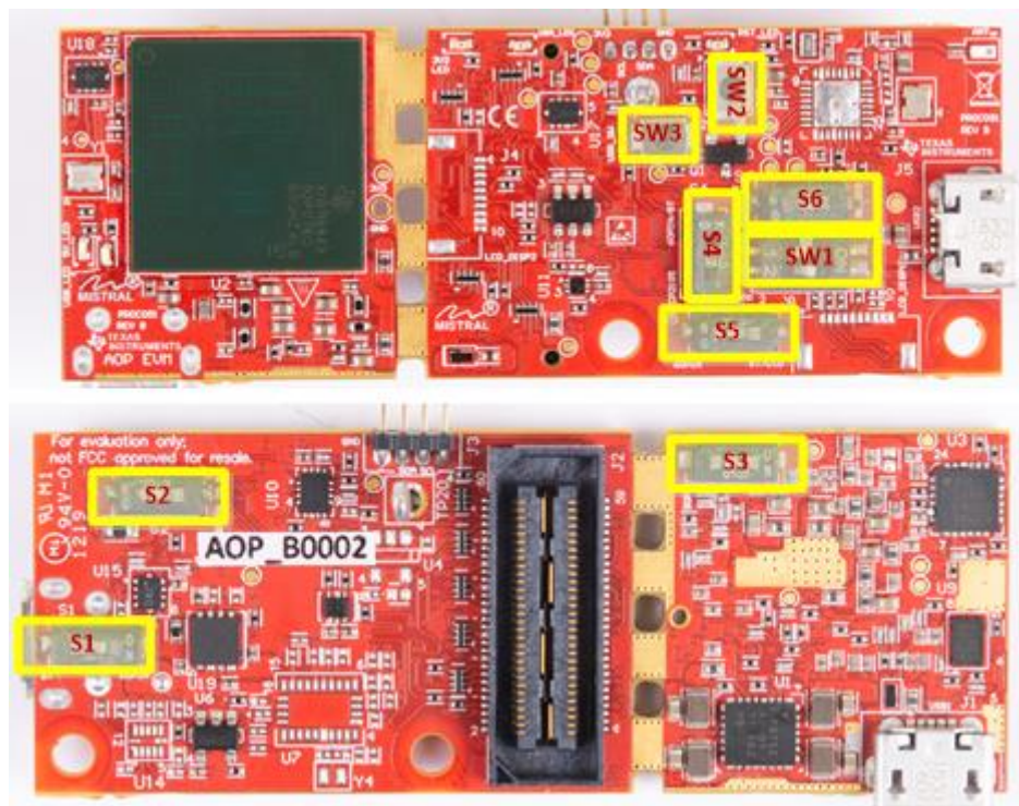
Figure 95. IWR6843AOPEVM Switches
