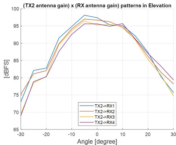
Figure 47. TX2 Antenna Radiation Pattern in Elevation
