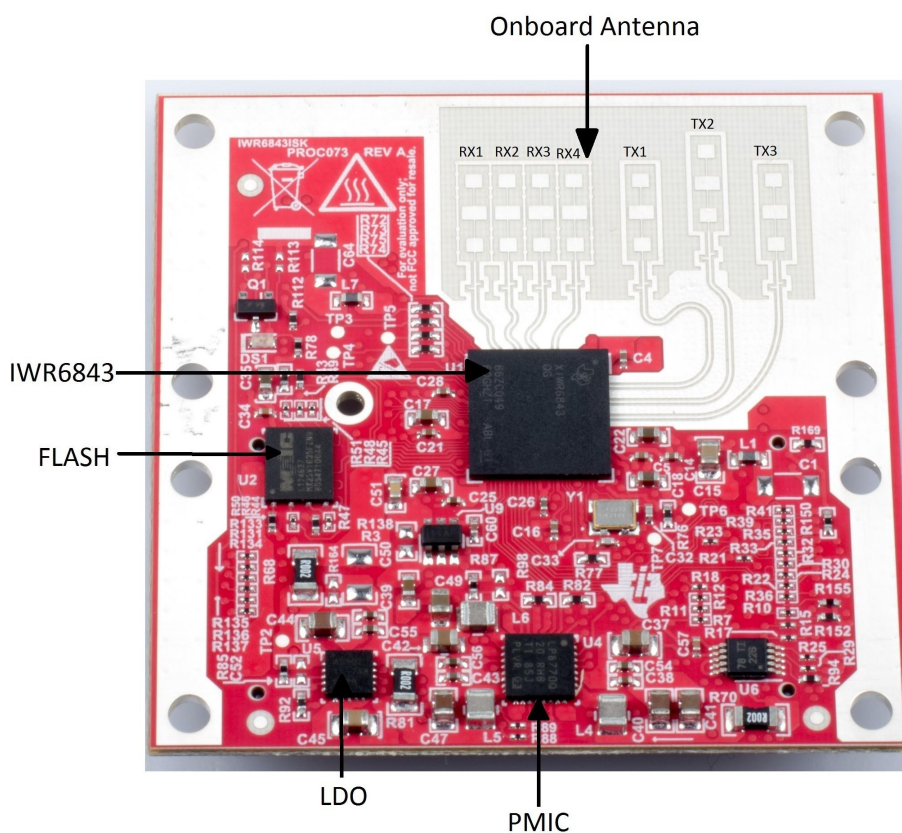
Figure 73. IWR6843ISK Front View
