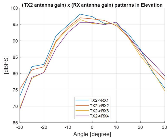
Figure 84. TX2 Antenna Radiation Pattern in Elevation
