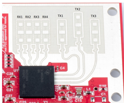
Figure 41. PCB Antennas
