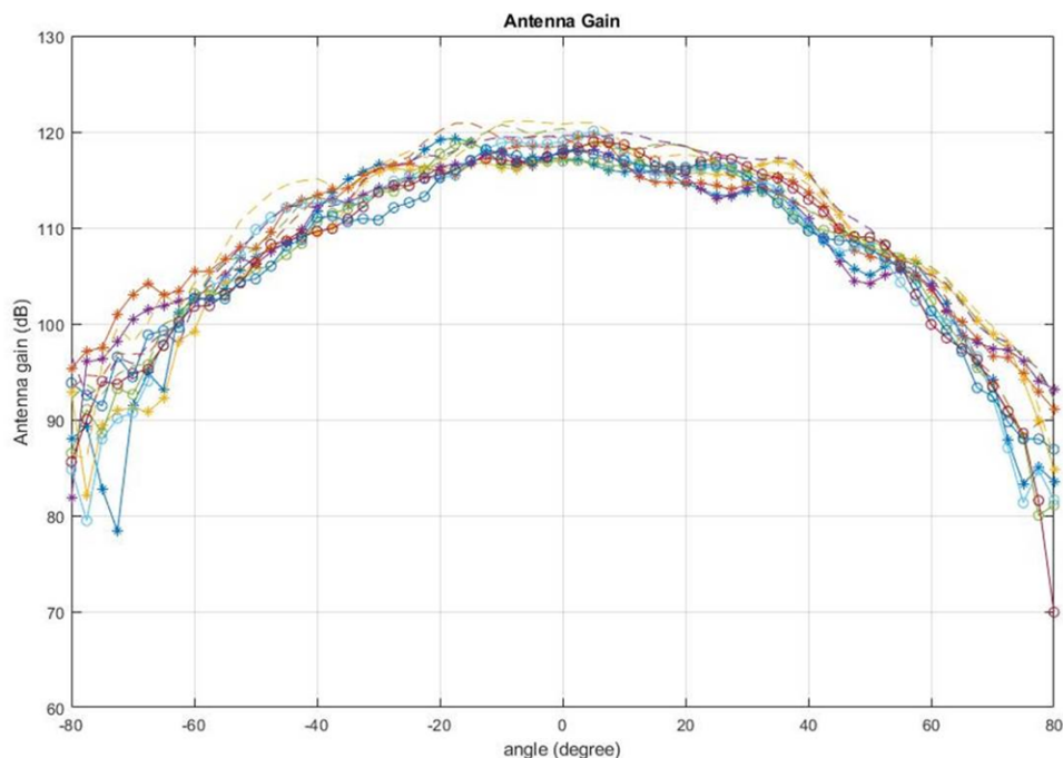
Figure 87. Measured Azimuthal Radiation Pattern for All Tx to Rx Pairs (All 12 Virtual Antenna Pairs Included)
