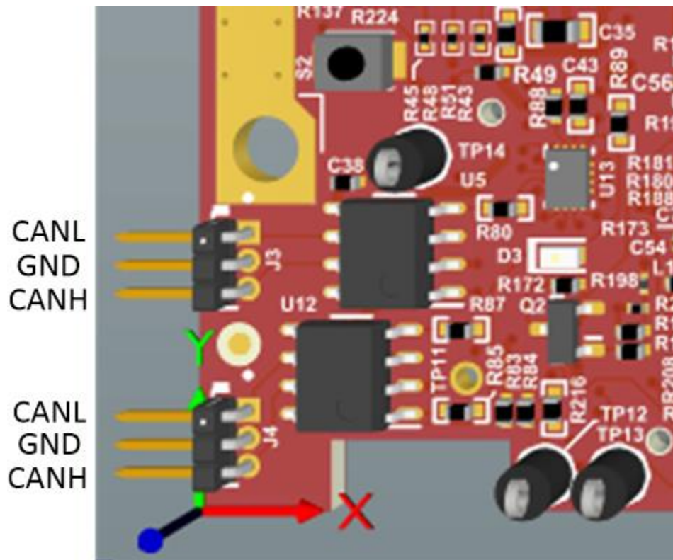
Figure 40. CAN Connector location and label
