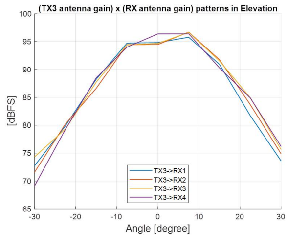
Figure 85. TX3 Antenna Radiation Pattern in Elevation
