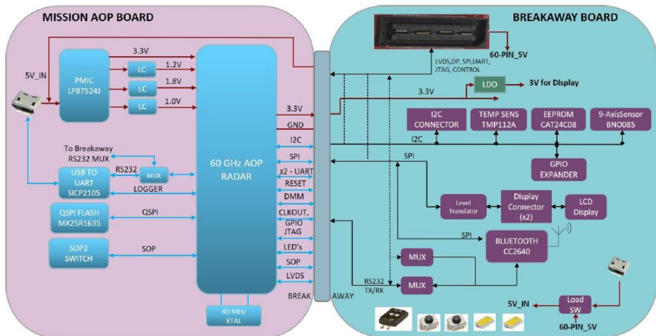
Figure 91. Block Diagram of the IWR6843AOPEVM
