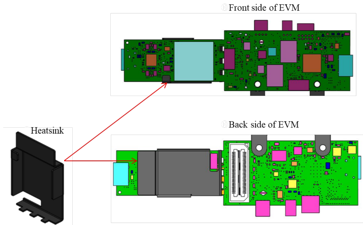
Figure 62. Heat sink placement
