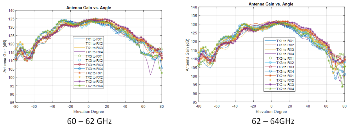
Figure 66. Measured Elevation Radiation Pattern for All Tx to Rx Pairs (All 12 Virtual Antenna Pairs Included)
