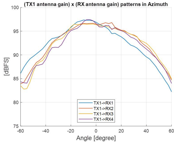
Figure 43. TX1 Antenna Radiation Pattern in Azimuth
