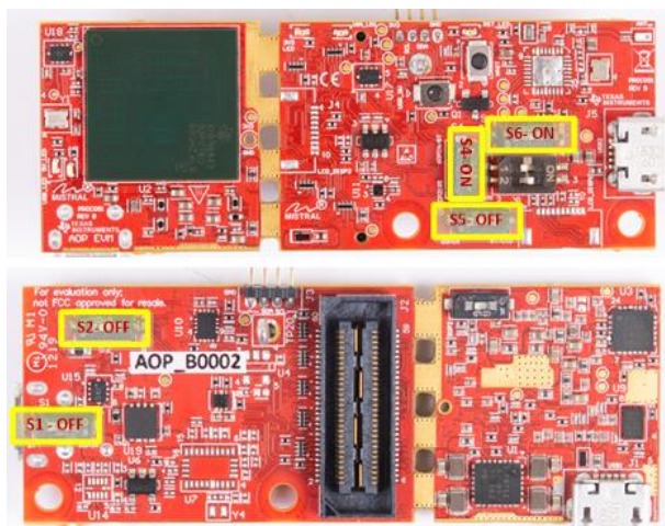
Figure 97. Switch Configuration for BT Mode
