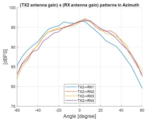
Figure 81. TX2 Antenna Radiation Pattern in Azimuth
