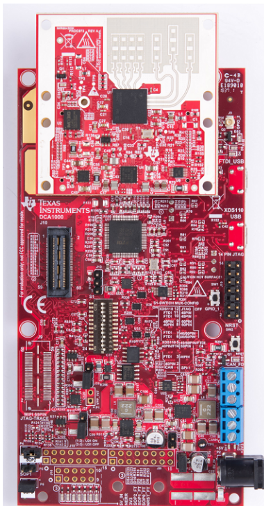
Figure 10. Integration of MMWAVEICBOOST and Starter Kit
