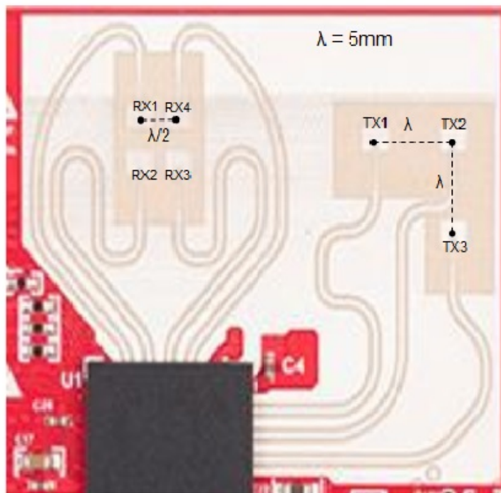
Figure 50. IWR6843ISK-ODS antenna placement MIMO array
