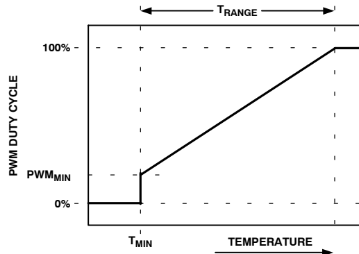
Figure 52. T_{\text{RANGE}} Parameter Affects Cooling Slope
