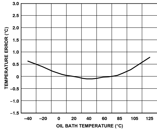
Figure 10. Internal Temperature Error vs. SCT221 Temperature
