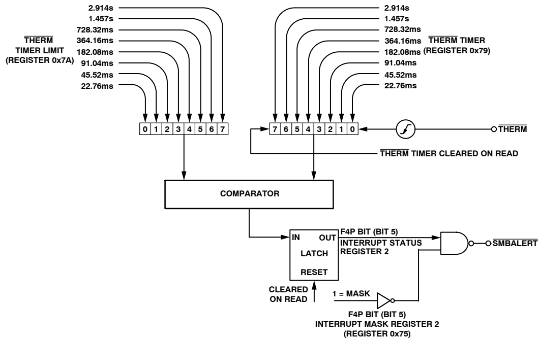
Figure 28. Functional Block Diagram of the SCT221 THERM Monitoring Circuitry
