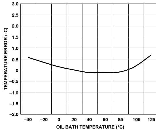
Figure 11. Remote Temperature Error vs. SCT221 Temperature
