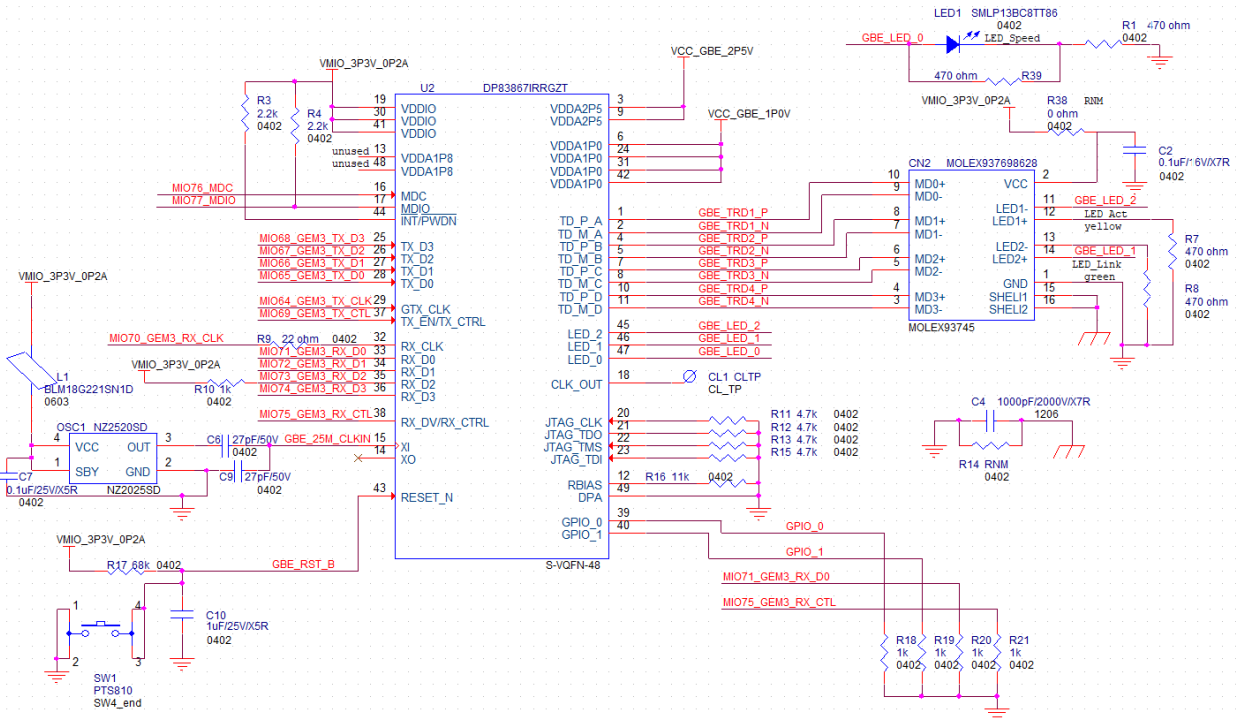
GigE board design (48-pin QFN RGZ package)
