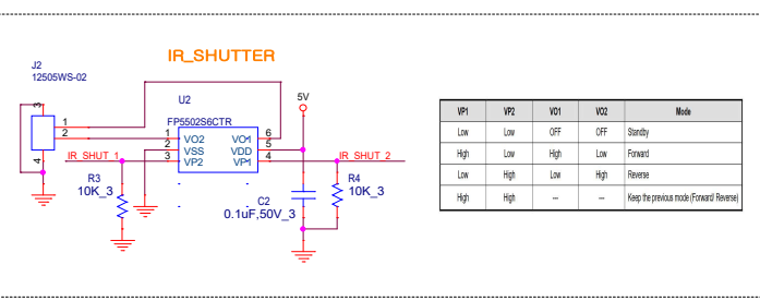
5V_IR
