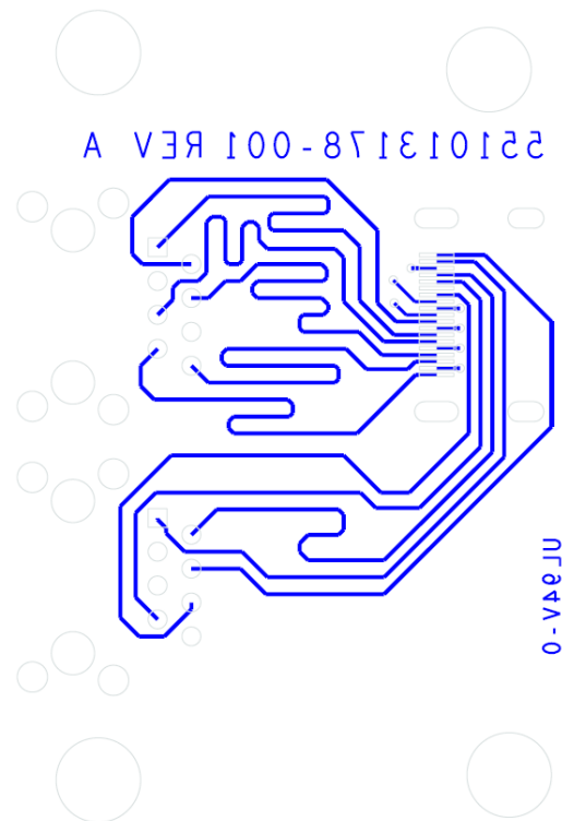
Bottom View
