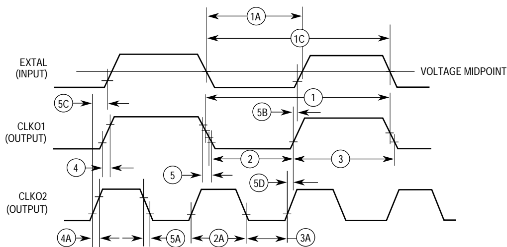
Figure 10-2. Clock Timing
