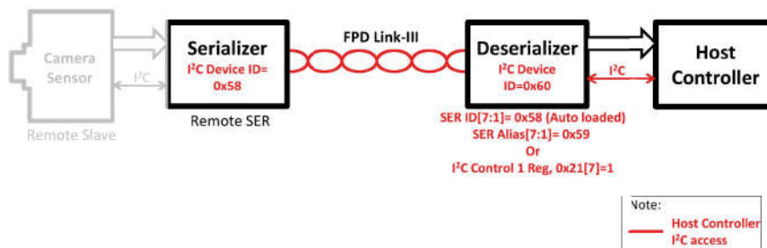
Figure 3. Communication with remote SER
