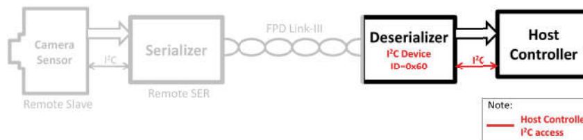
Figure 2. Local I 2 C
