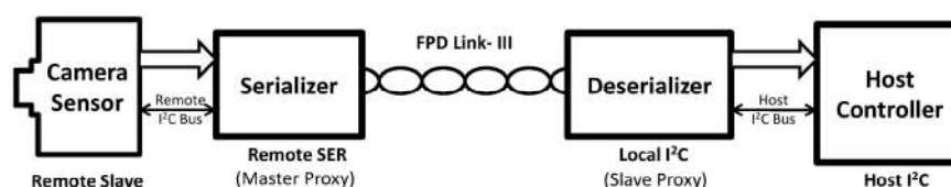
Figure 1. Typical FPD-Link III Connection with I 2 C Bus
