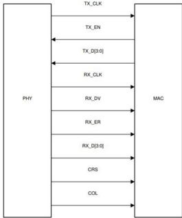
Figure 9-4. MII Signaling
