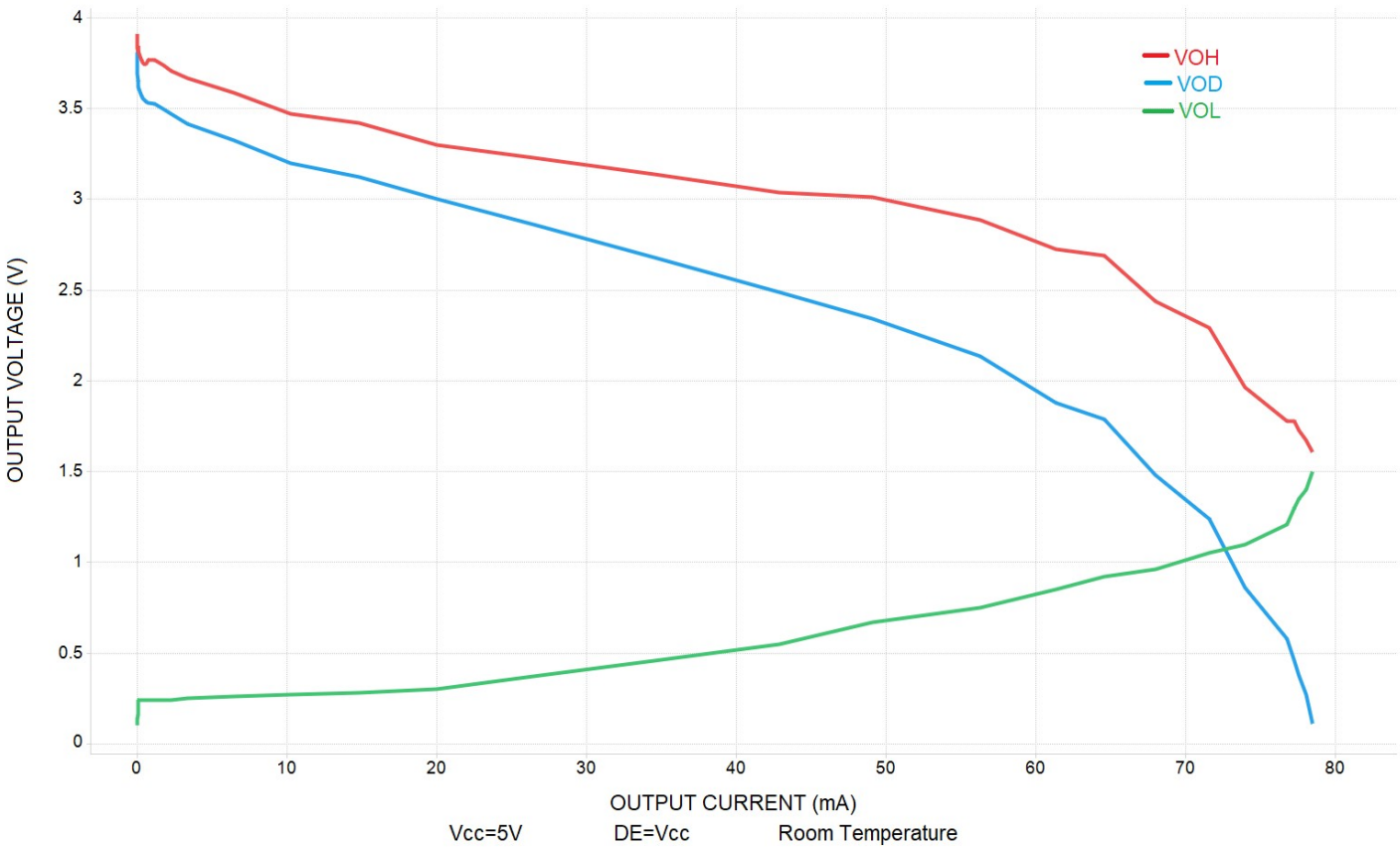
Driver Output voltage vs Driver Output Current
