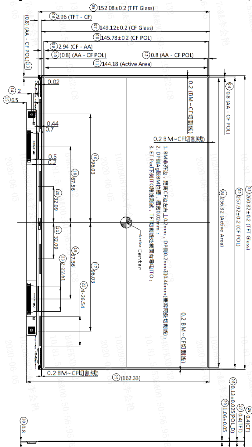
Figure 5. TFT-LCD FOB Outline Dimension (Front View)
