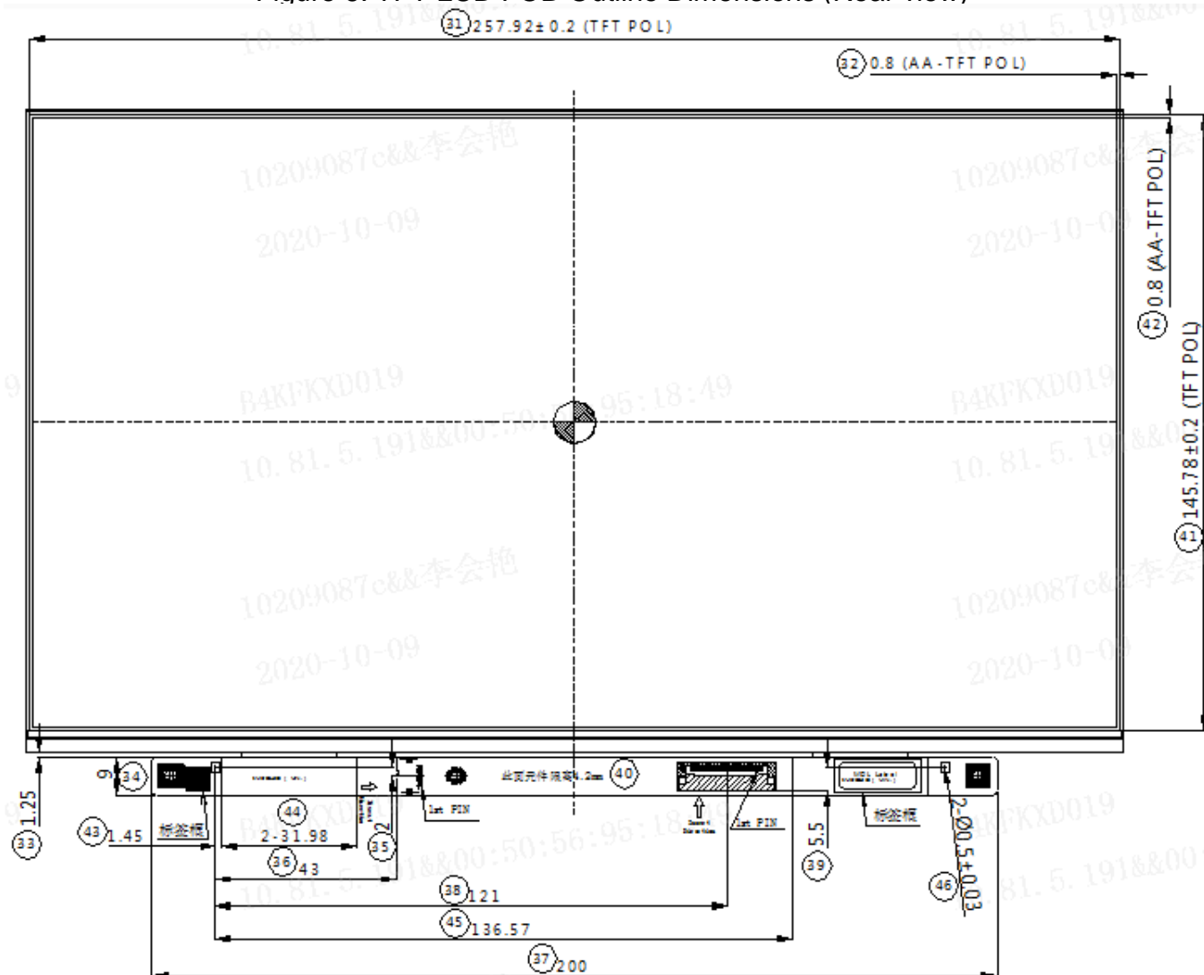
Figure 6. TFT-LCD FOB Outline Dimensions (Rear view)
