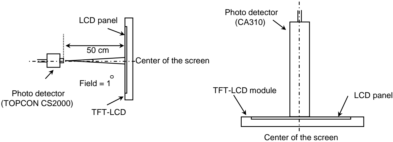
View angel range, etc. measurement setup
