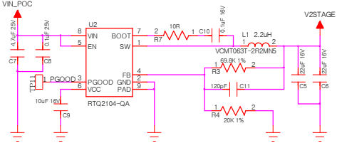
Step Down Conv. 5V-> 3.6V/3A For LDO
