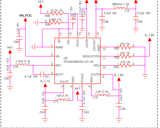
SENSOR_POWER
