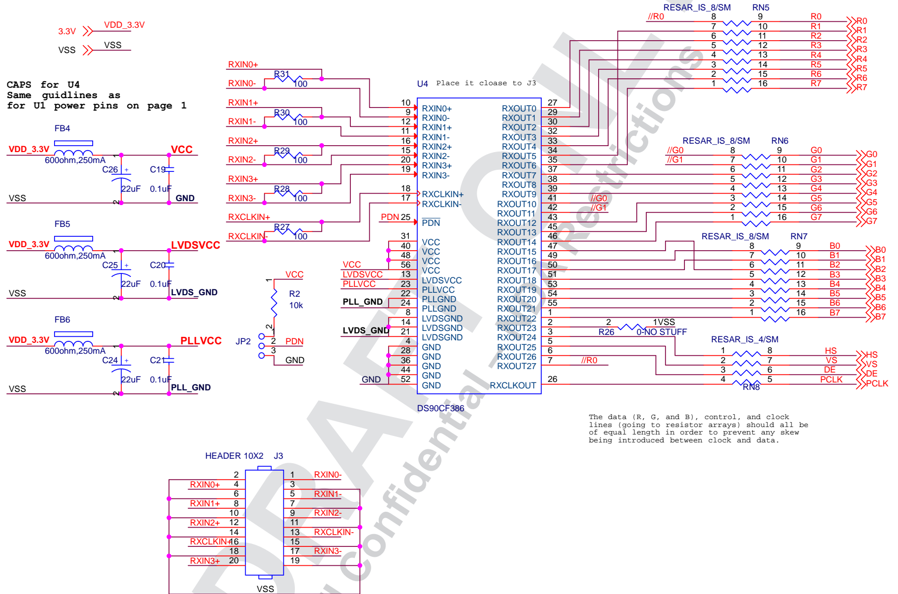
Figure A-2. LVDS Receiver: DS90CF386
