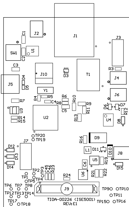
Figure 37. Top Assembly
