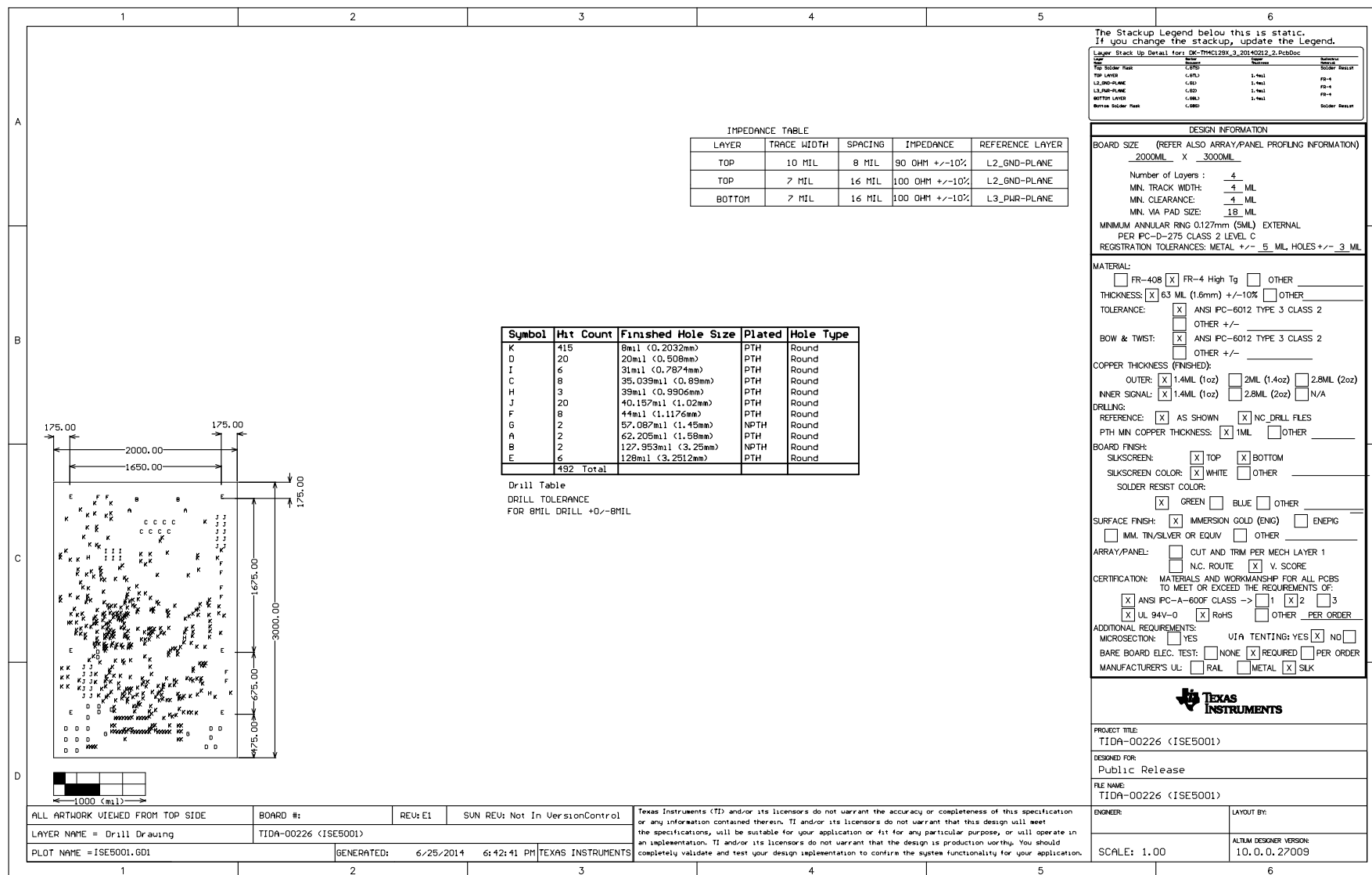
Figure 34. Fabrication Drawing
