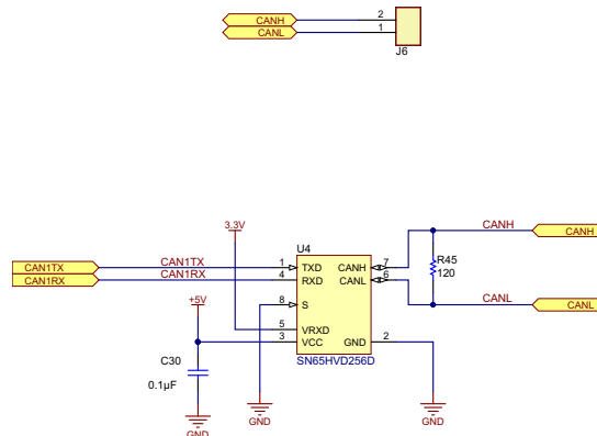
Figure 5. CAN Interface
