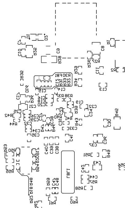
Figure 31. Bottom Overlay
