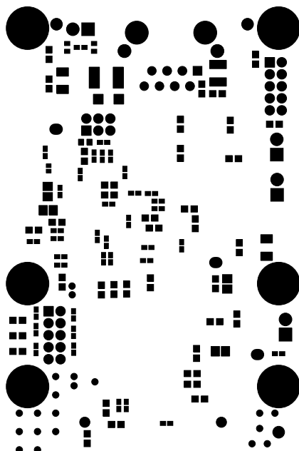
Figure 30. Bottom Soldermask
