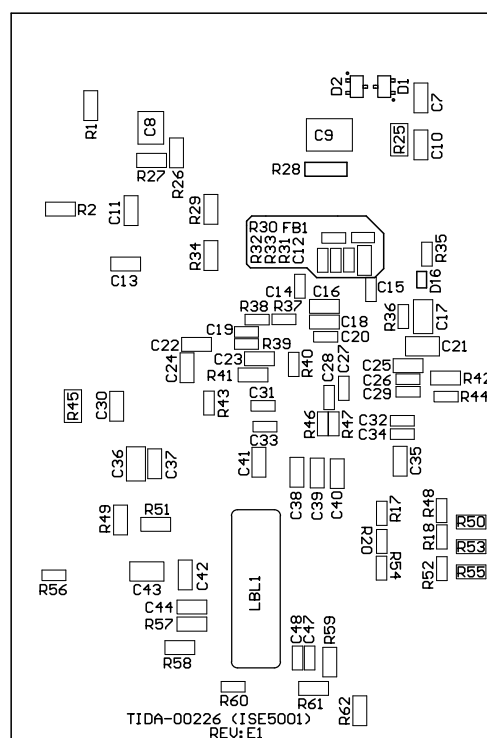
Figure 38. Bottom Assembly
