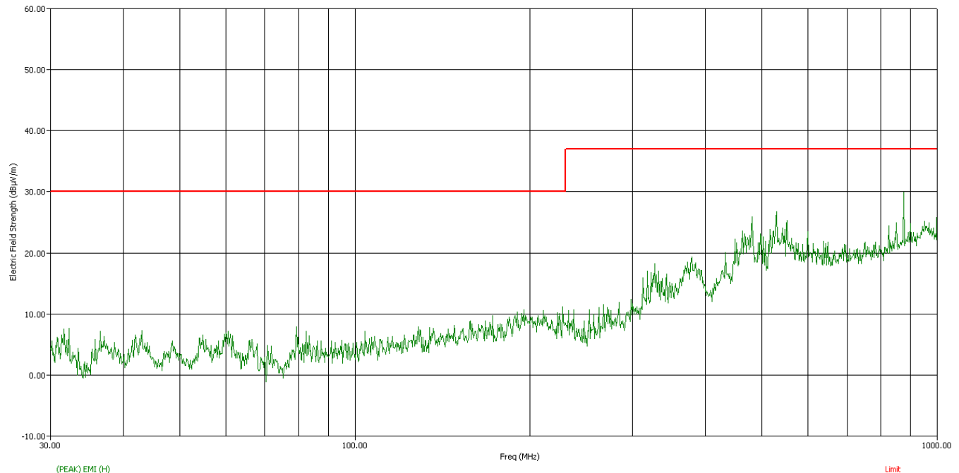
Figure 16. Horizontal Polarization
