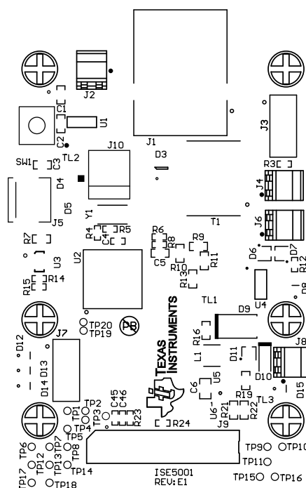
Figure 25. Top Overlay
