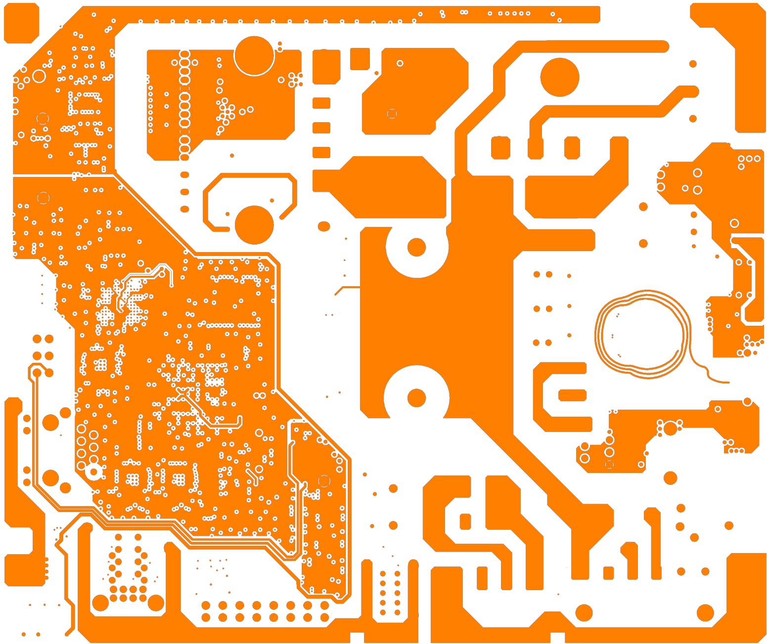
#5 POWER LAYER5
