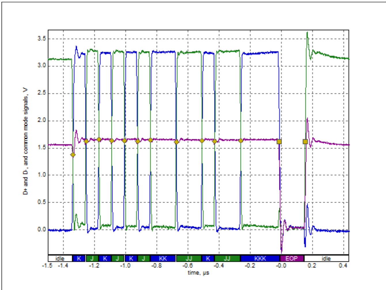
Scope Capture Data Plot, Path on Scope: D:\Applications\USB2\Results\FSUpstreamSQ955Plot.png Timestamp: 12/14/2022 13:17:45
