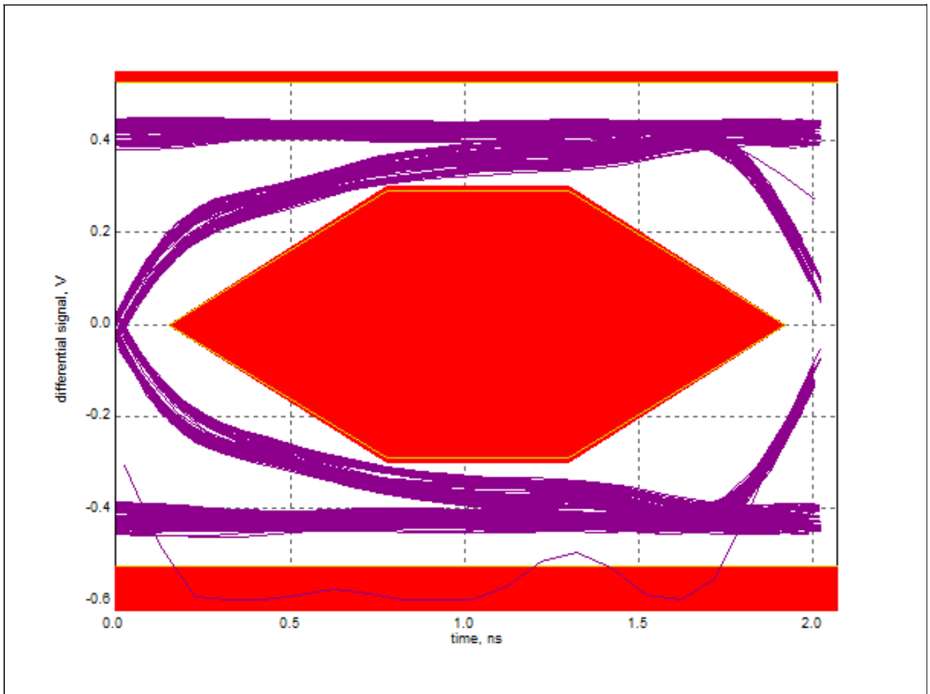
Upstream Eye Diagram, Path on Scope: D:\Applications\USB2\Results\HSUpstreamSQ517Eye.png Timestamp: 12/14/2022 11:12:54
