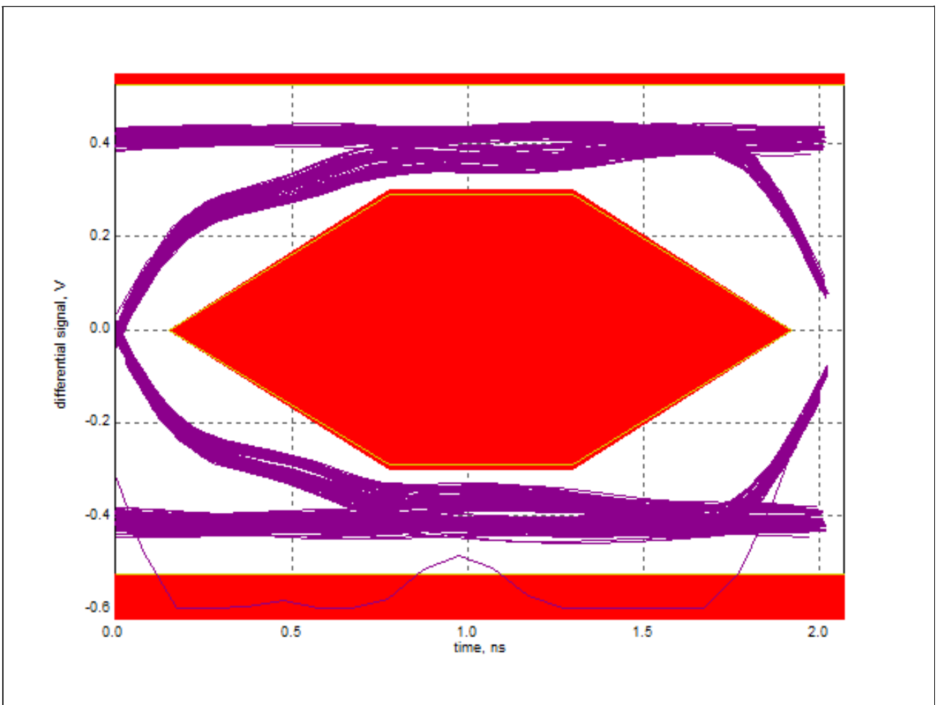
Upstream Eye Diagram, Path on Scope: D:\Applications\USB2\Results\HSJitter5Eye.png Timestamp: 12/14/2022 15:41:20
