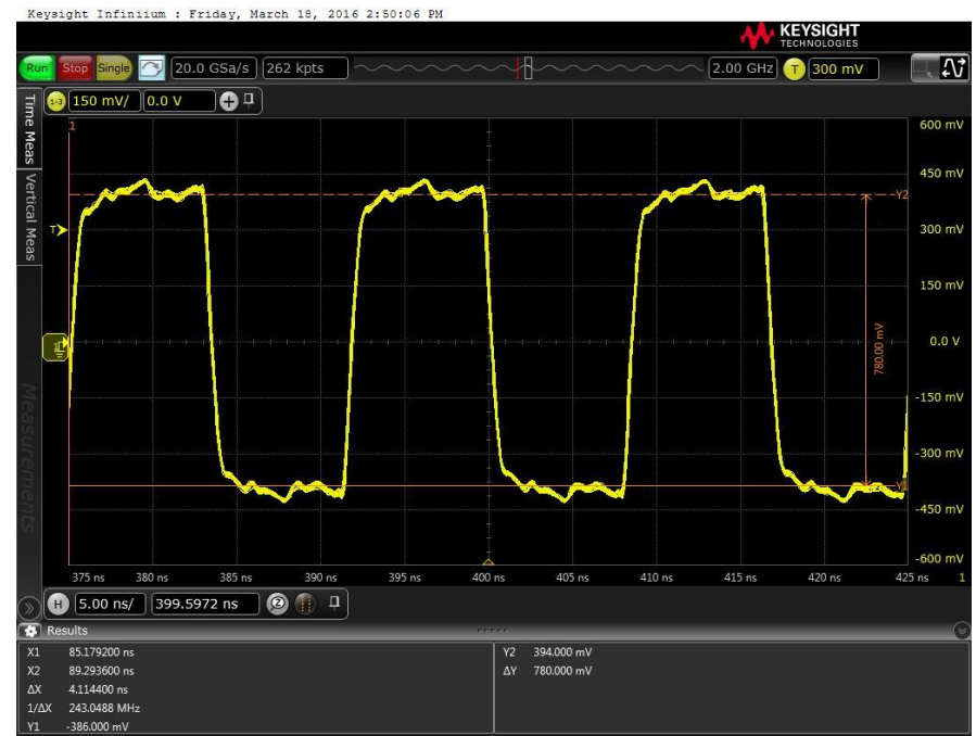
Fig. 2: Test Package without TUSB211
