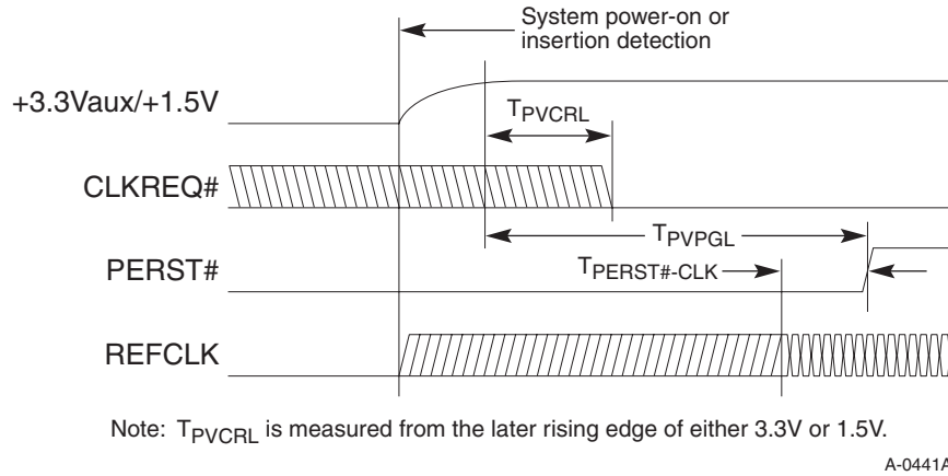
Figure 3-1: Power-Up CLKREQ# Timing
