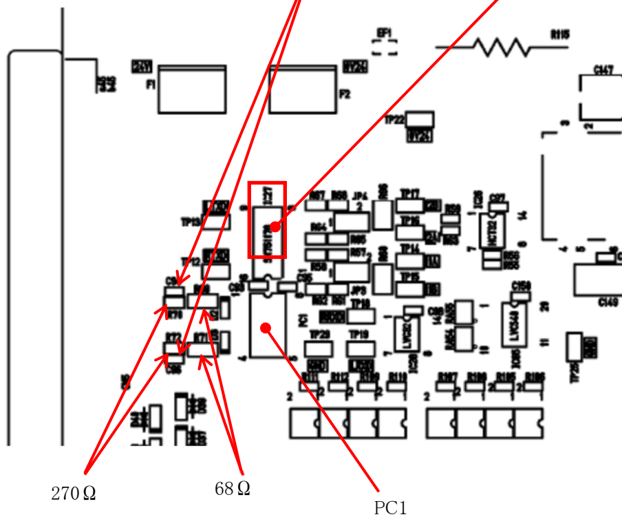
< Board mounted state: printed circuit board silk printing >
