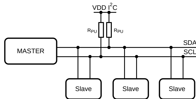
Figure 1. Example of I²C Bus
