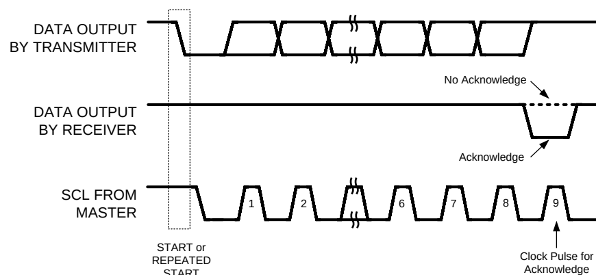
Figure 2. Acknowledge On The I²C Bus
