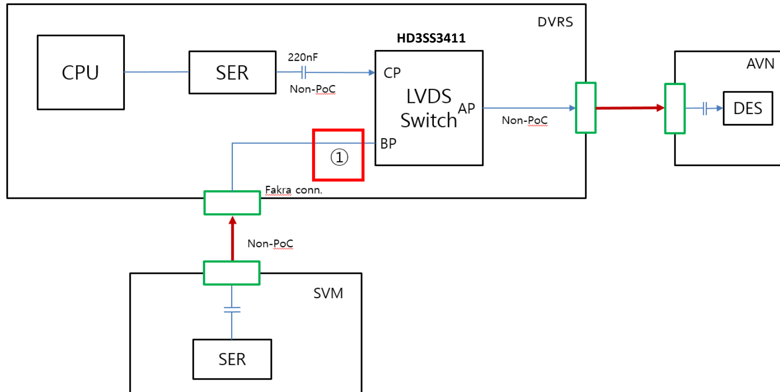
Signal flow block of HD3SS3411
