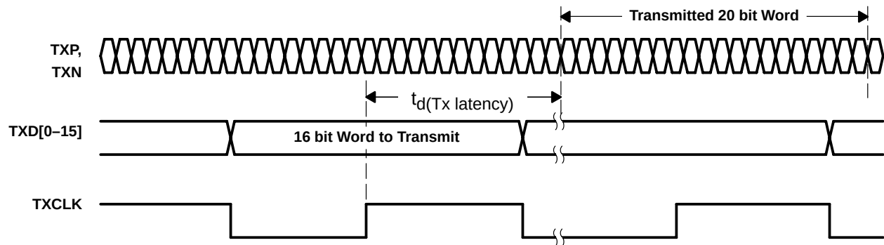
Figure 3. Transmitter Latency
