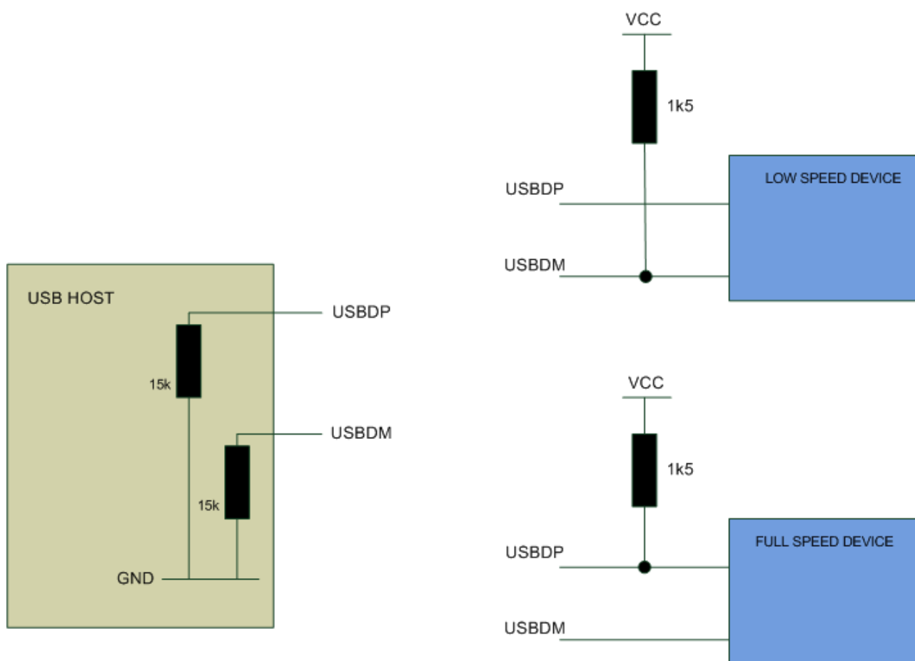
Figure 1: Connection of low / full speed devices.
