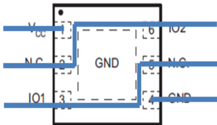
DRS PACKAGE (TOP VIEW)
