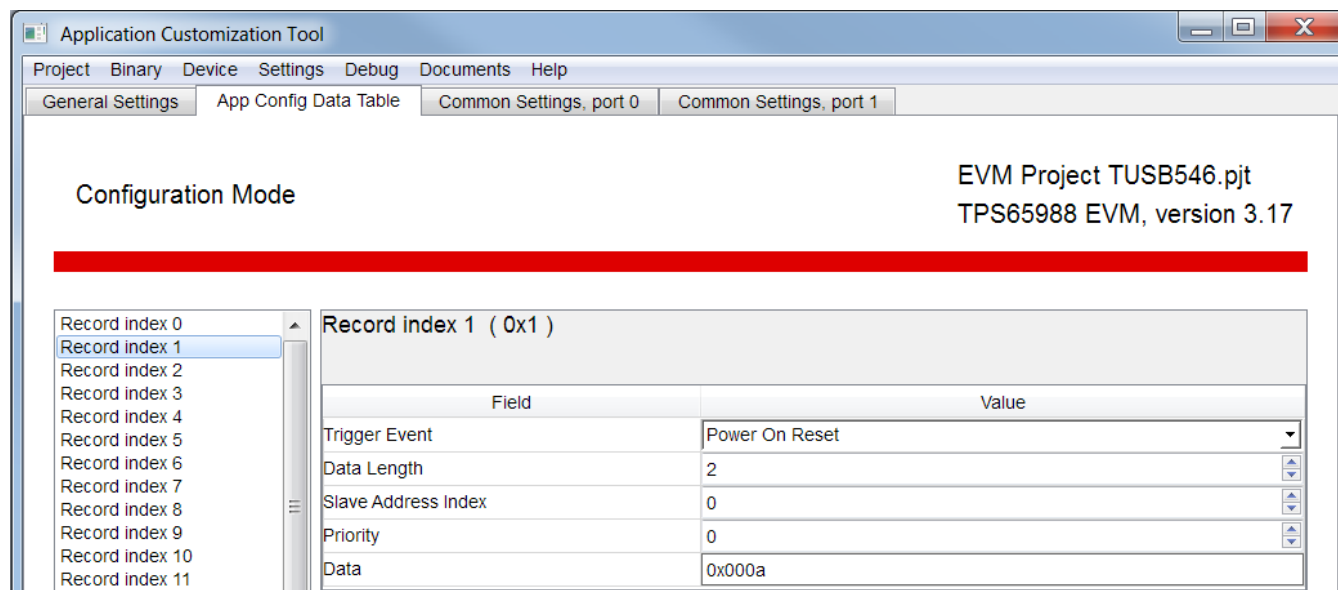
Figure 13. Power Up Data for TUSB546
