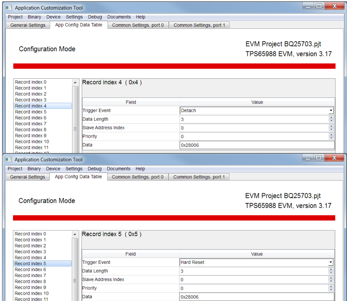
Figure 9. Configuration for Hard Reset and Detach events
