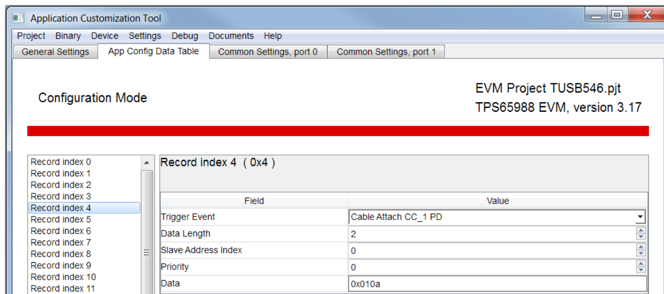
Figure 14. Configuration Data for TUSB546
