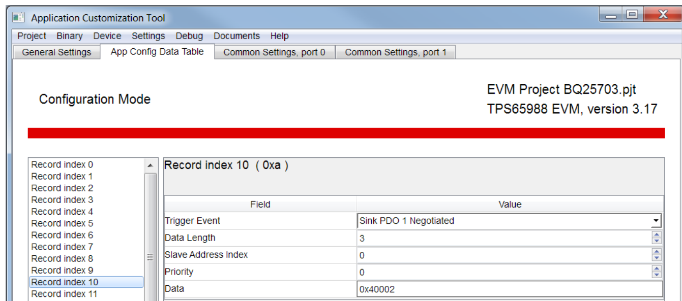
Figure 10. Record Index for 5 V Sink PDO
