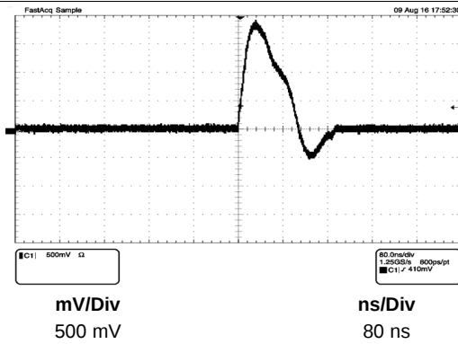
Figure 14. 10Base-Tc Link Pulse
