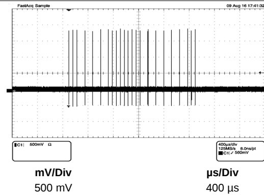
Figure 15. Auto-Negotiation FLP
