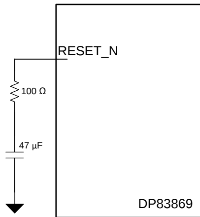
Figure 32. RESET_N Circuit
