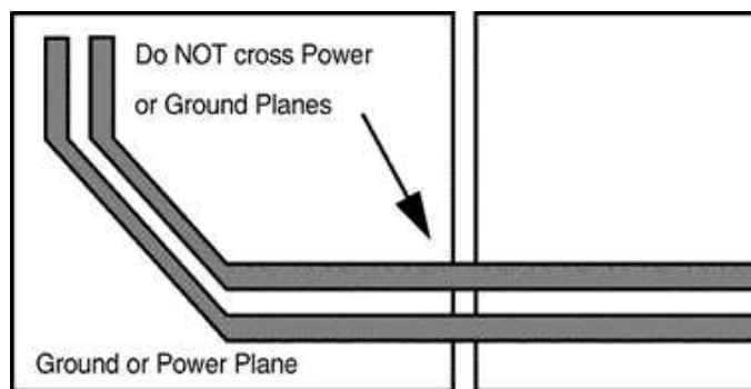
Figure 119. Differential Signal Pair-Plane Crossing
