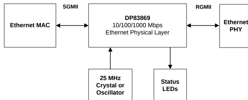
Figure 3. SGMII-RGMII Bridge System Block Diagram
