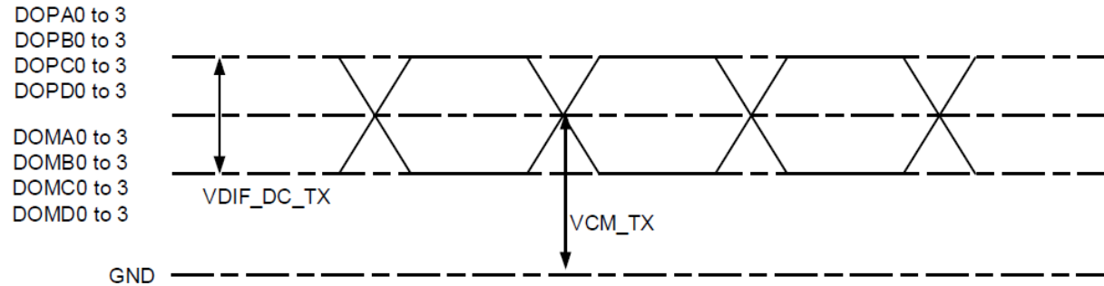
Fig. DC output of TX of SLVS-EC
