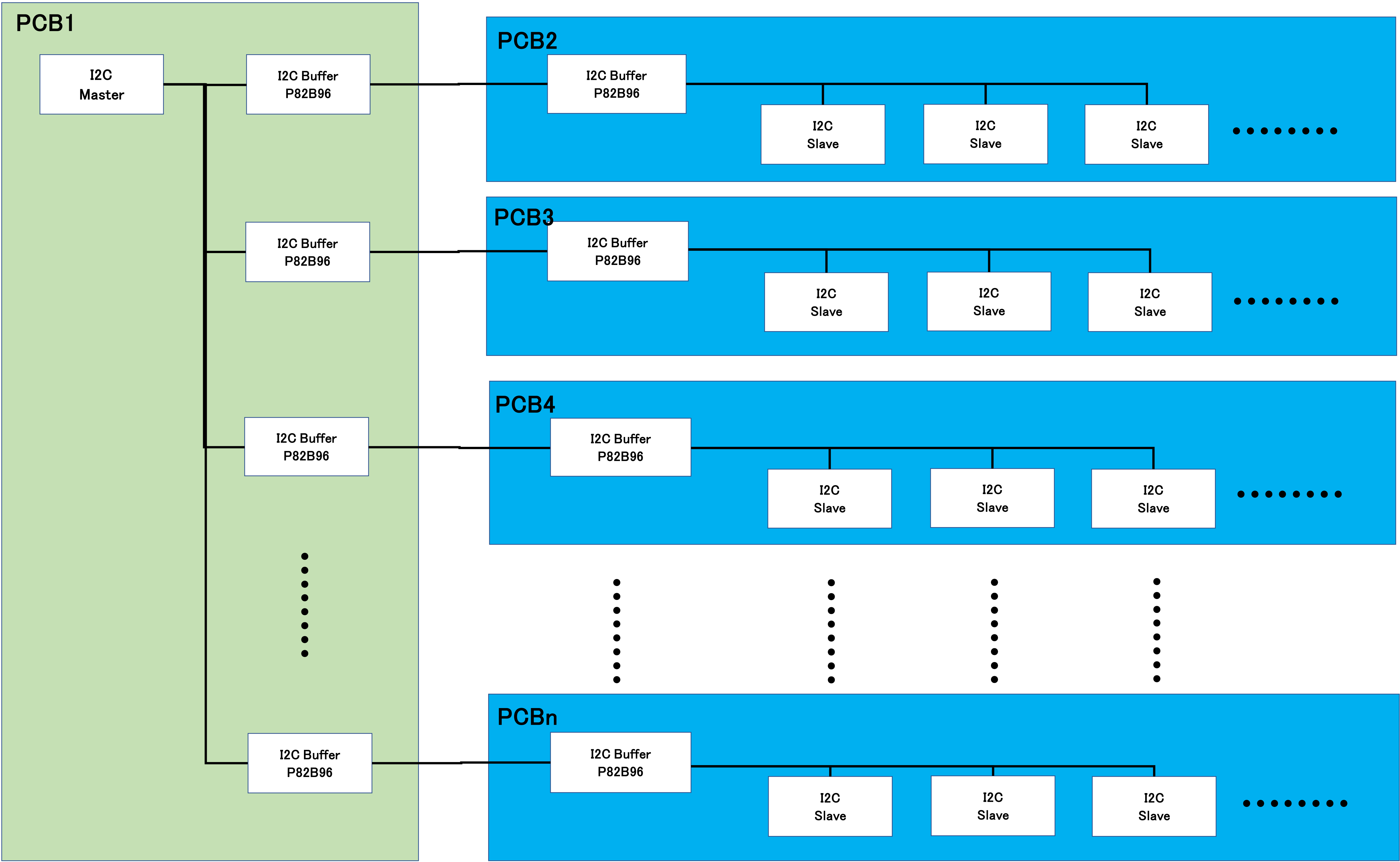
Connection Diagram
