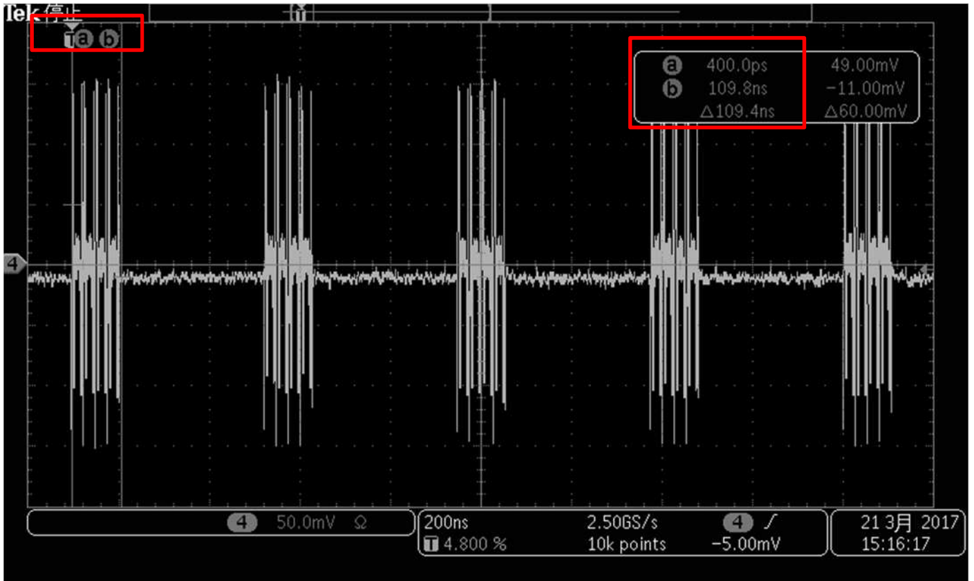
CPU output
