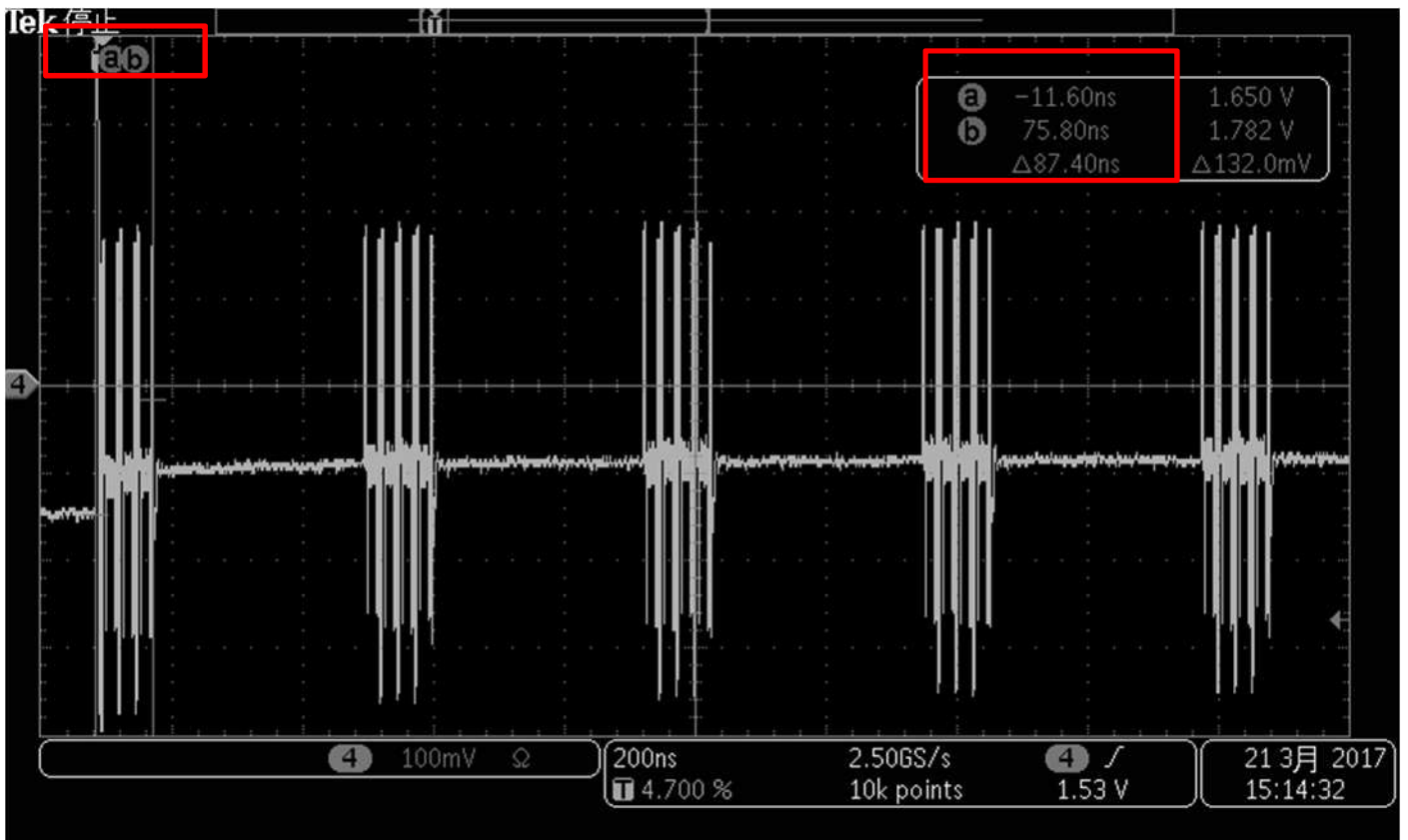
Repeater Output(SN75LVCP600S)
