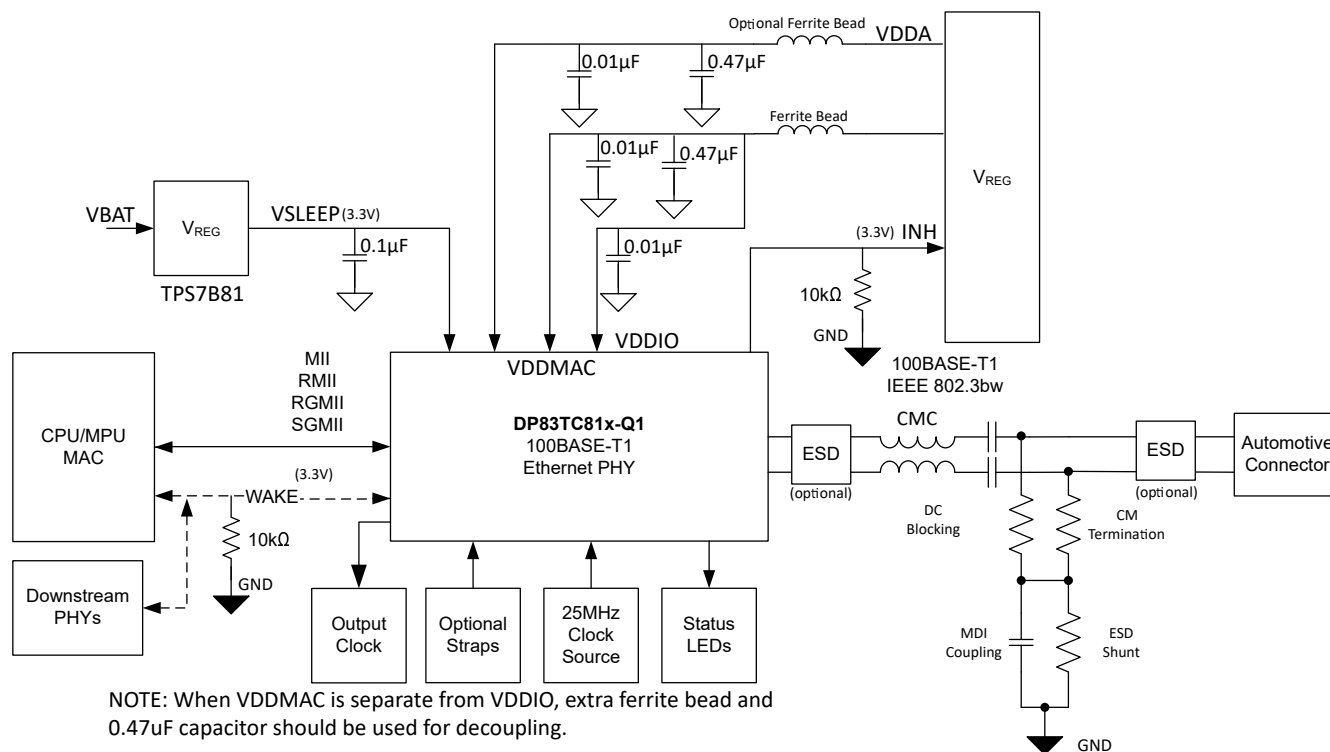
Figure 2-5. Typical TC-10 Application With Peripheral (DP83TC812 and DP83TC813)
