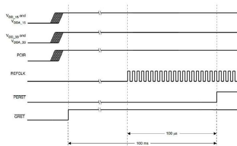
Figure 4. Power-Up Sequence
