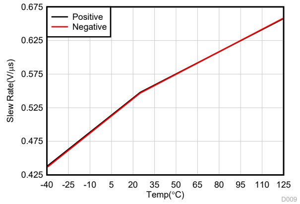
Figure 7-34. Slew Rate vs Temperature
