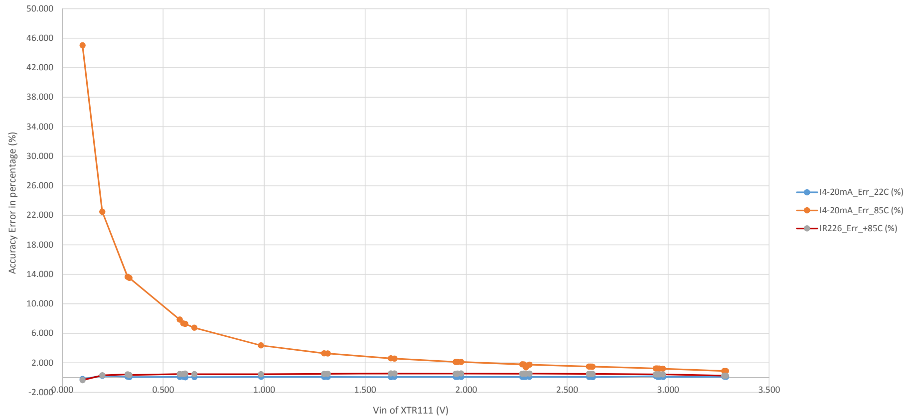
Accuracy of 4-20mA current at +22C and +85C compared with theoretical calculation
