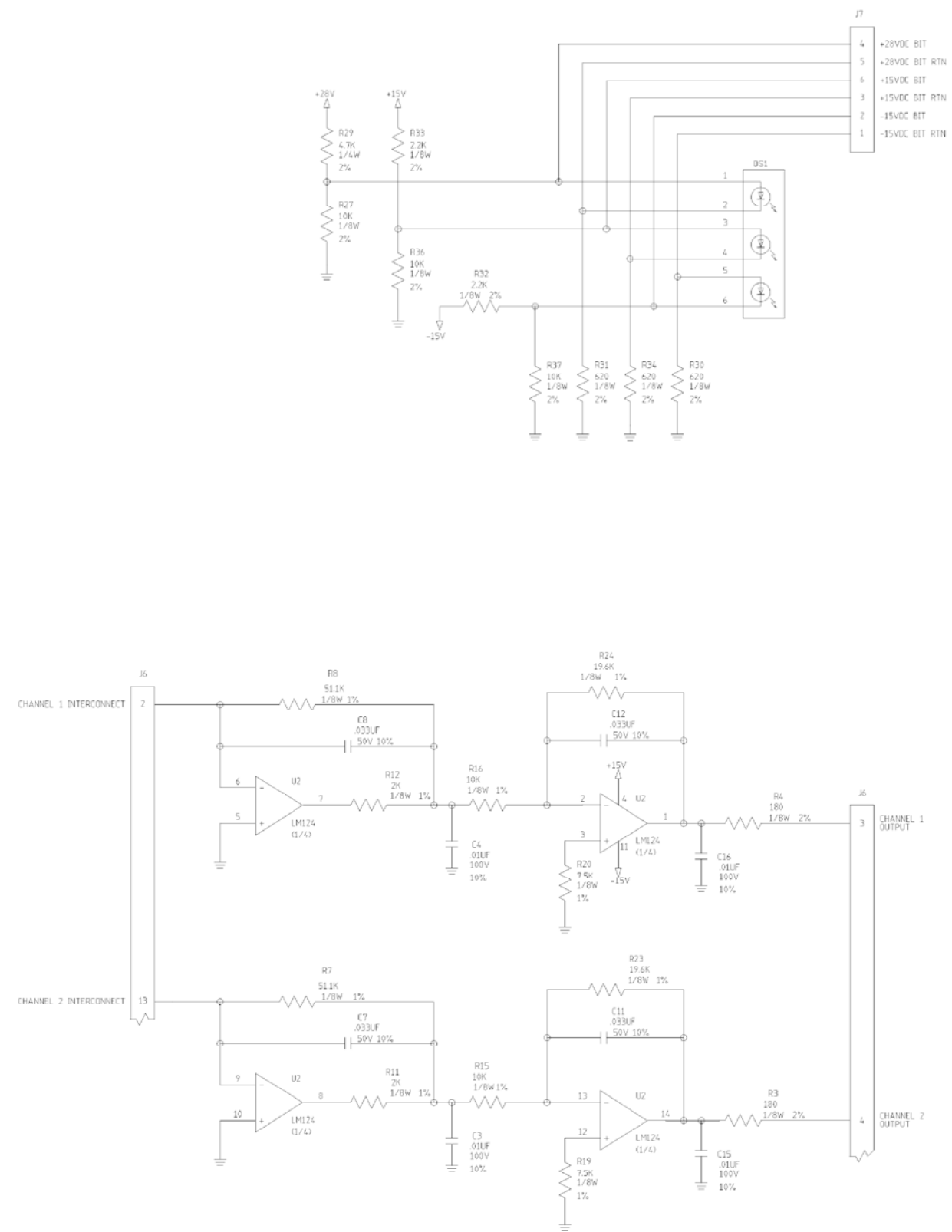
-11 SCHEMATIC
