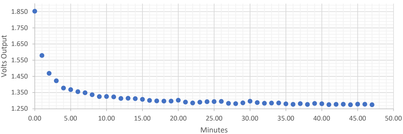
Test #41 INA333 Vref = 1.1978 volts
