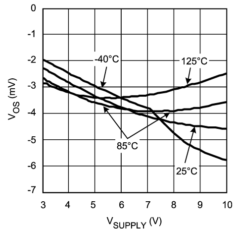
V_{\text{OS}} vs. V_{\text{SUPPLY}} for Unit 2
