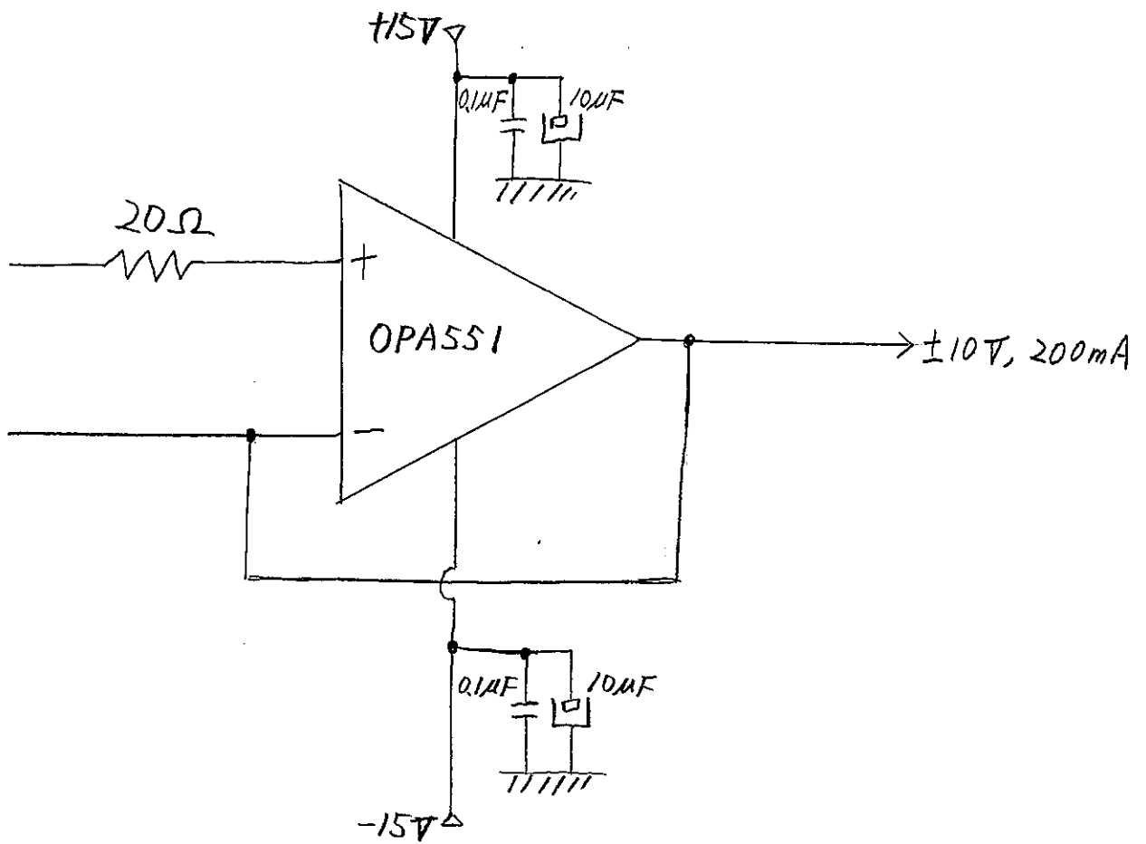
Figure 1. Customer circuit
