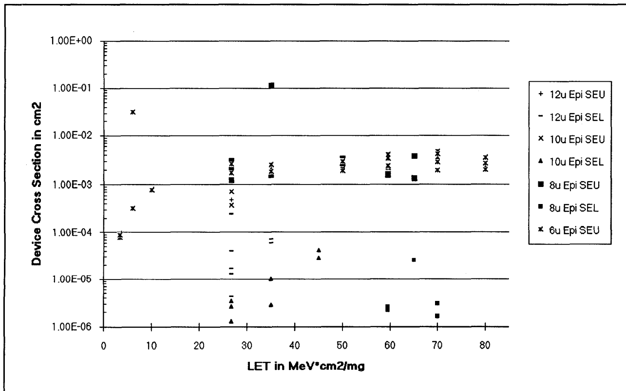
Figure 5 7201 SEU/SEL Comparison, Device Cross Sections
