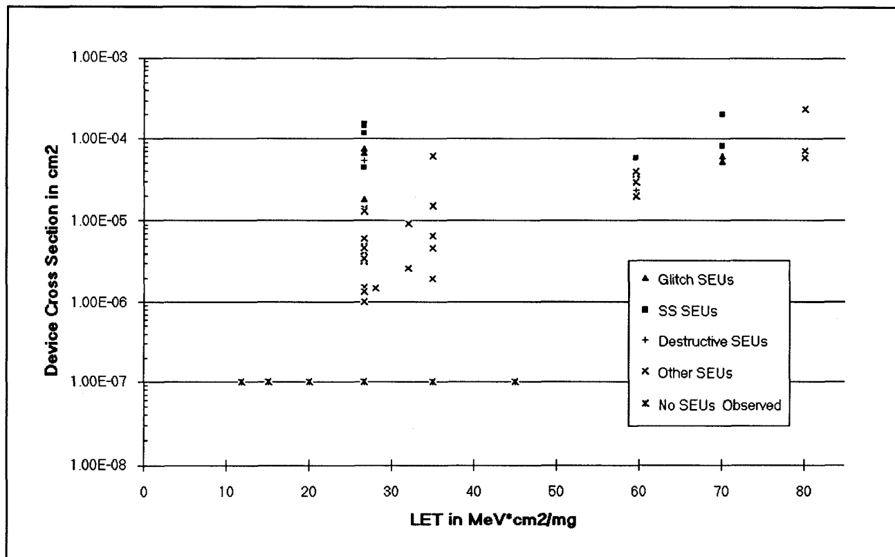
Figure 2 AHE2815, Device Cross Sections
