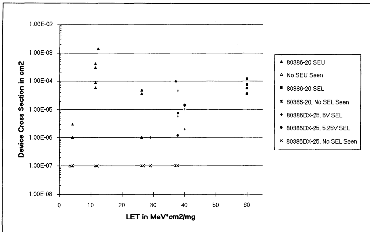
Figure 6 80386 SEU/SEL, Device Cross Sections
