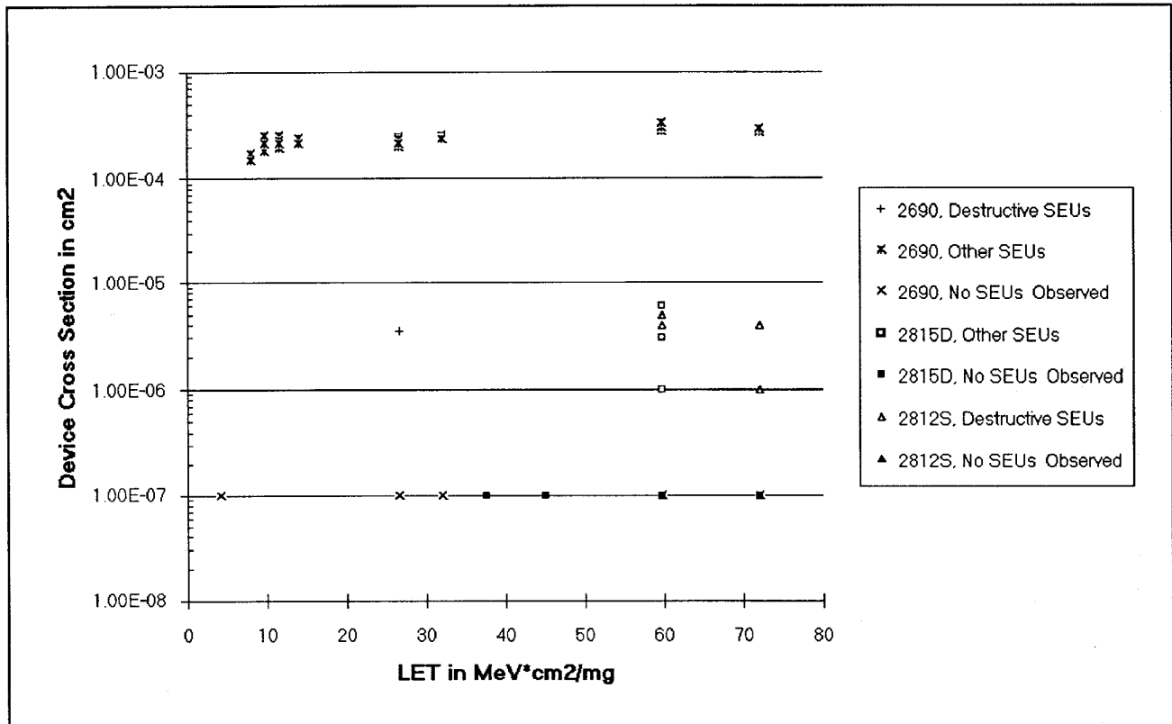
Figure 3 DC/DC Converters, Device Cross Sections
