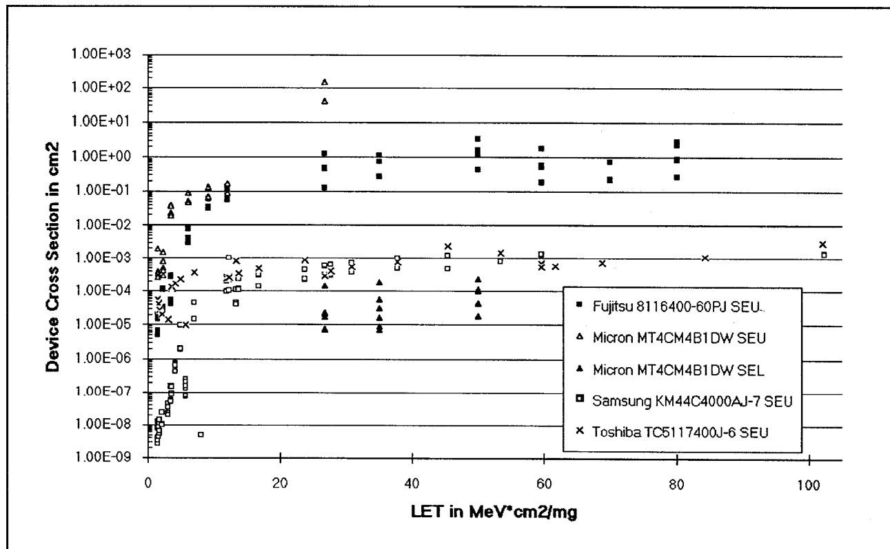
Figure 4 DRAM SEU/SEL, Device Cross Sections
