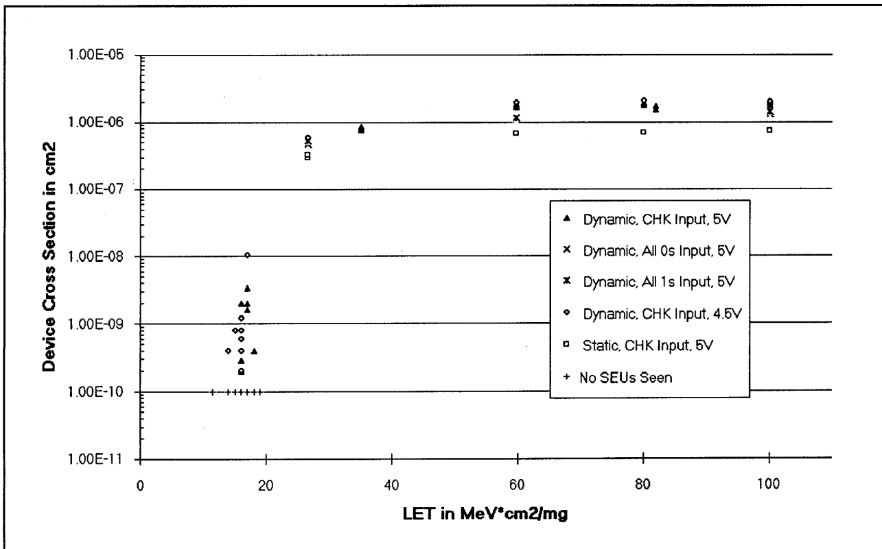
Figure 8 HR2340 Honeywell Test Metal, Cross Sections per Flip-Flop
