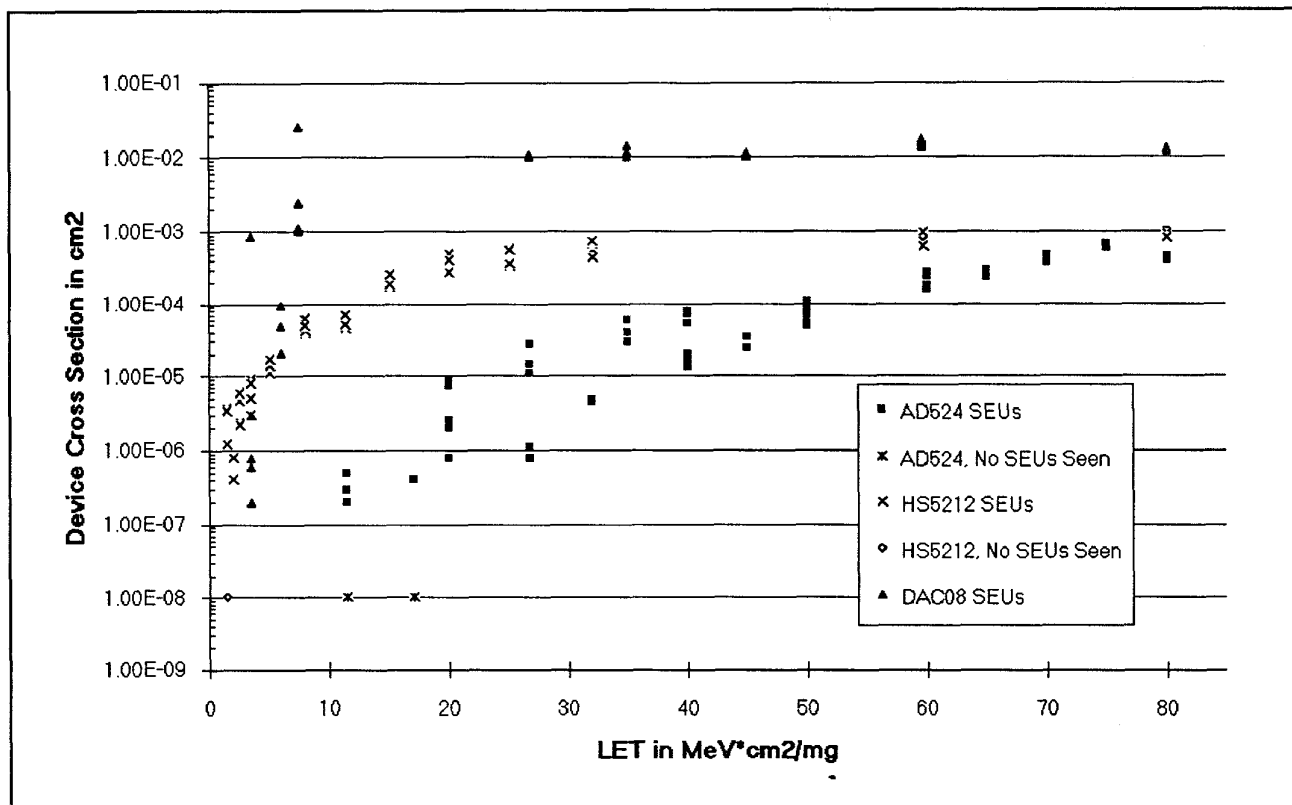
Figure 1 Analog Devices, Device Cross Sections
