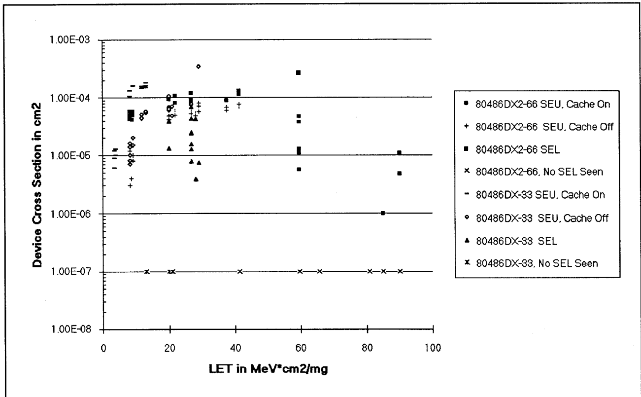
Figure 7 80486 SEU/SEL, Device Cross Sections
