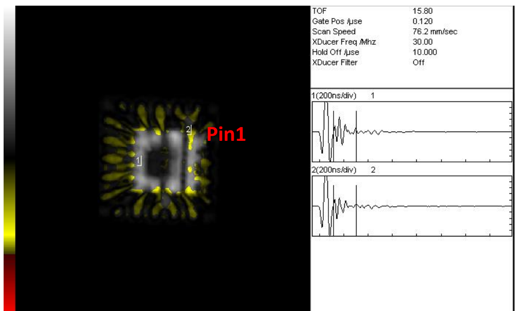
Fig.3: C-SAM image of returned unit. No delamination was observed over die surface.
