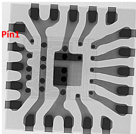
Fig.2: X-ray image of returned unit. No internal package issue was observed.
