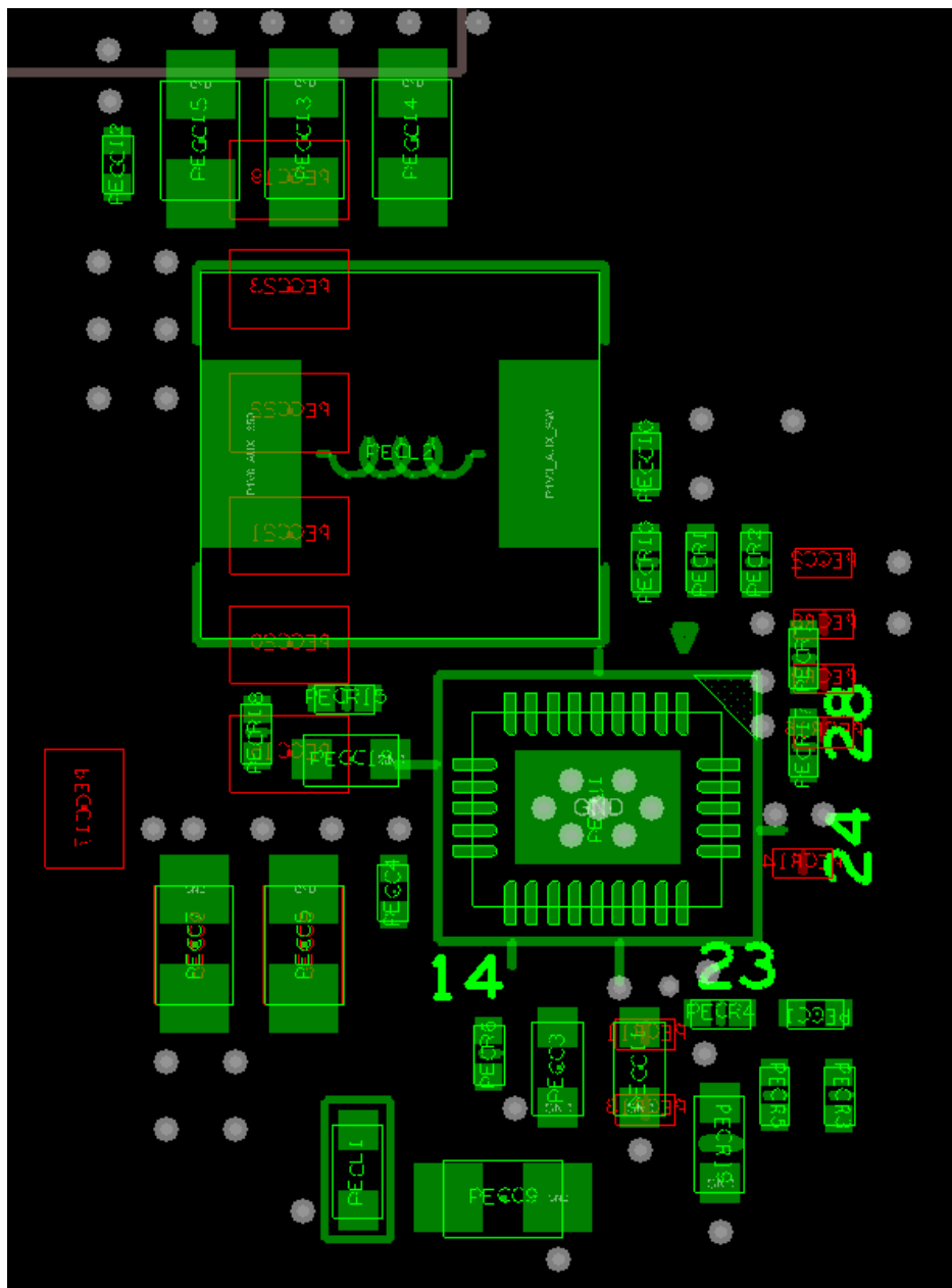
TOP placement
