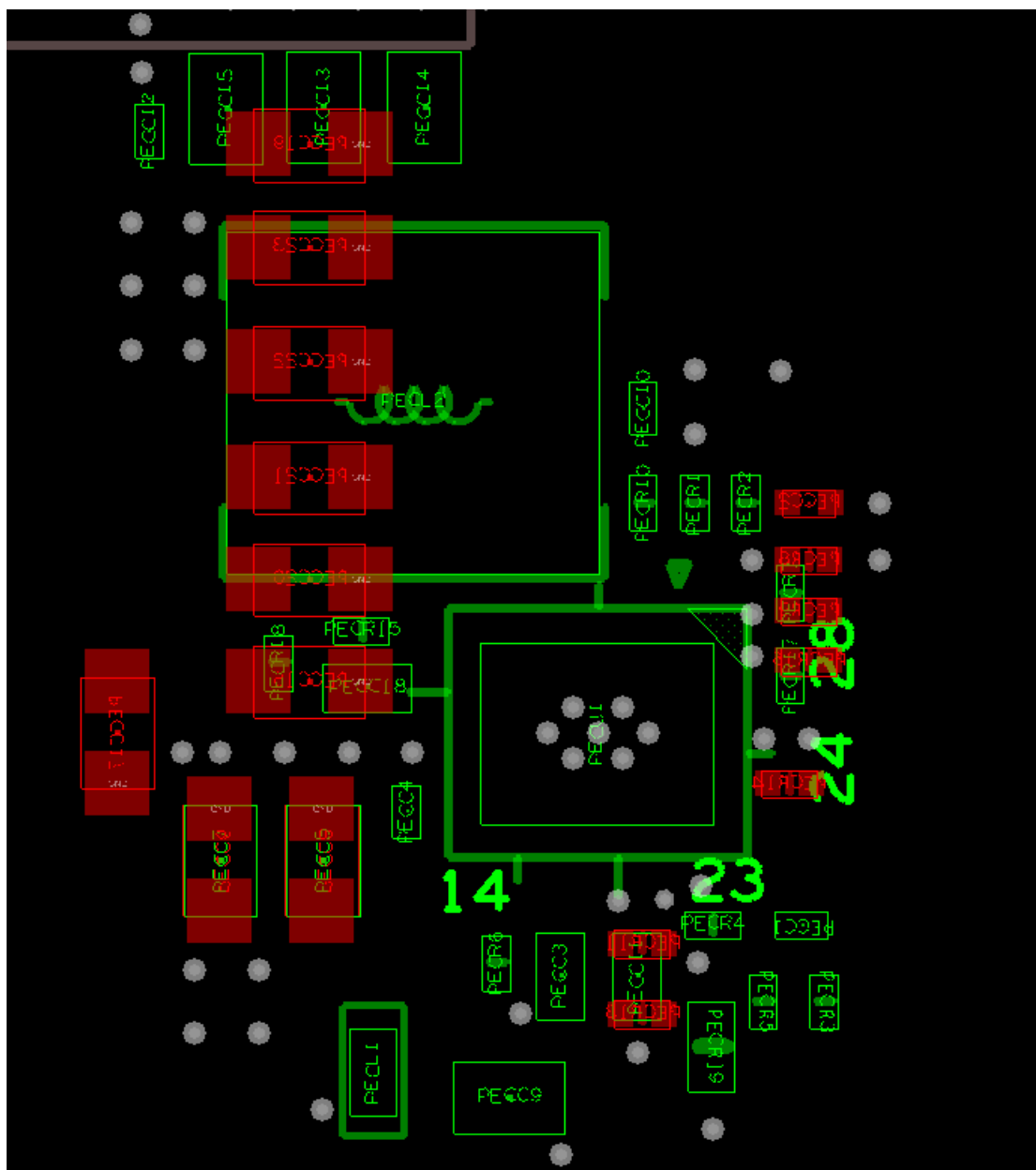
Bottom Placement
