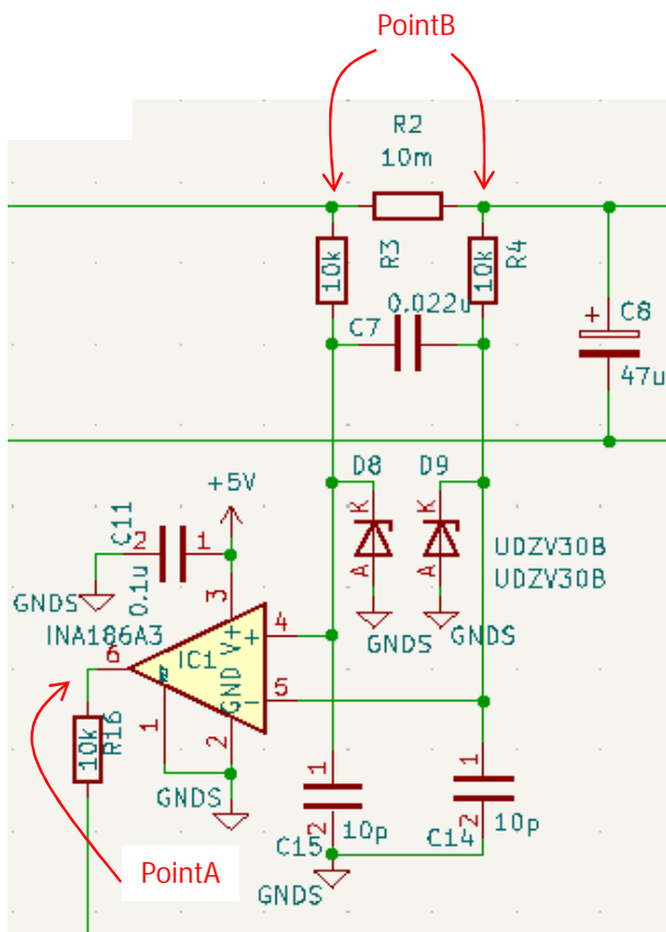
FIG1. CIRCUIT
