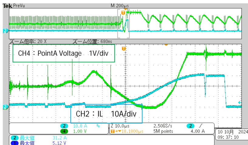
FIG3. Waveform2_Amp output
