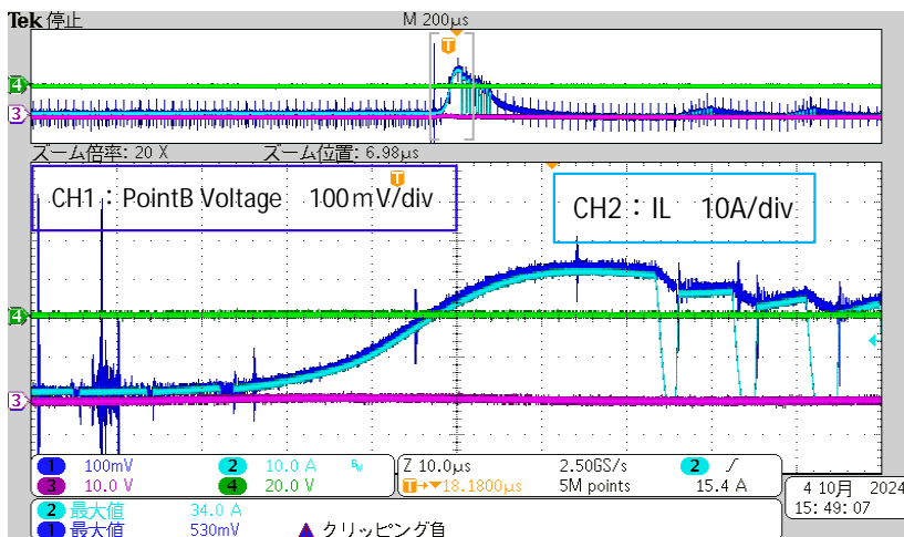
FIG2. Waveform1_Voltage across the shunt resistor
