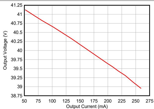
Figure 6-2. Output Voltage vs Output Current
