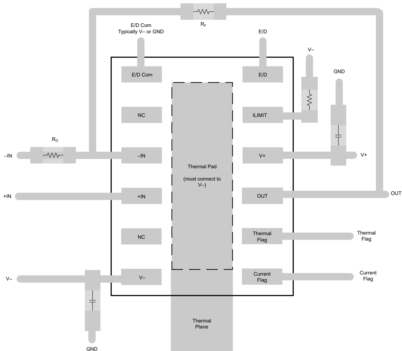
Figure 10-2. OPA593 Board Layout for Noninverting Configuration
