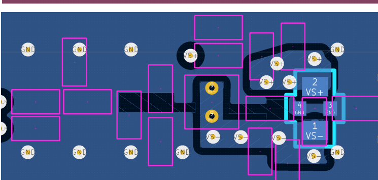
layer6 (bottom)
