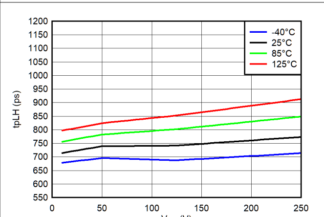
Figure 6-24. T_{PLH} vs Input Underdrive @ V_{CC} = 5.0\text{ V}
