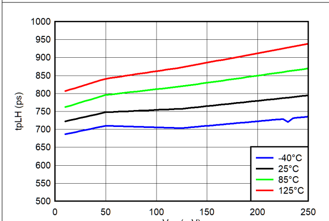
Figure 6-23. T_{PLH} vs Input Underdrive @ V_{CC} = 3.3\text{ V}
