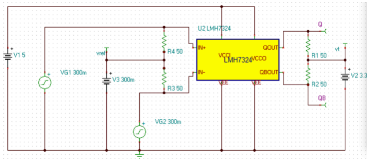
Simulation circuit
