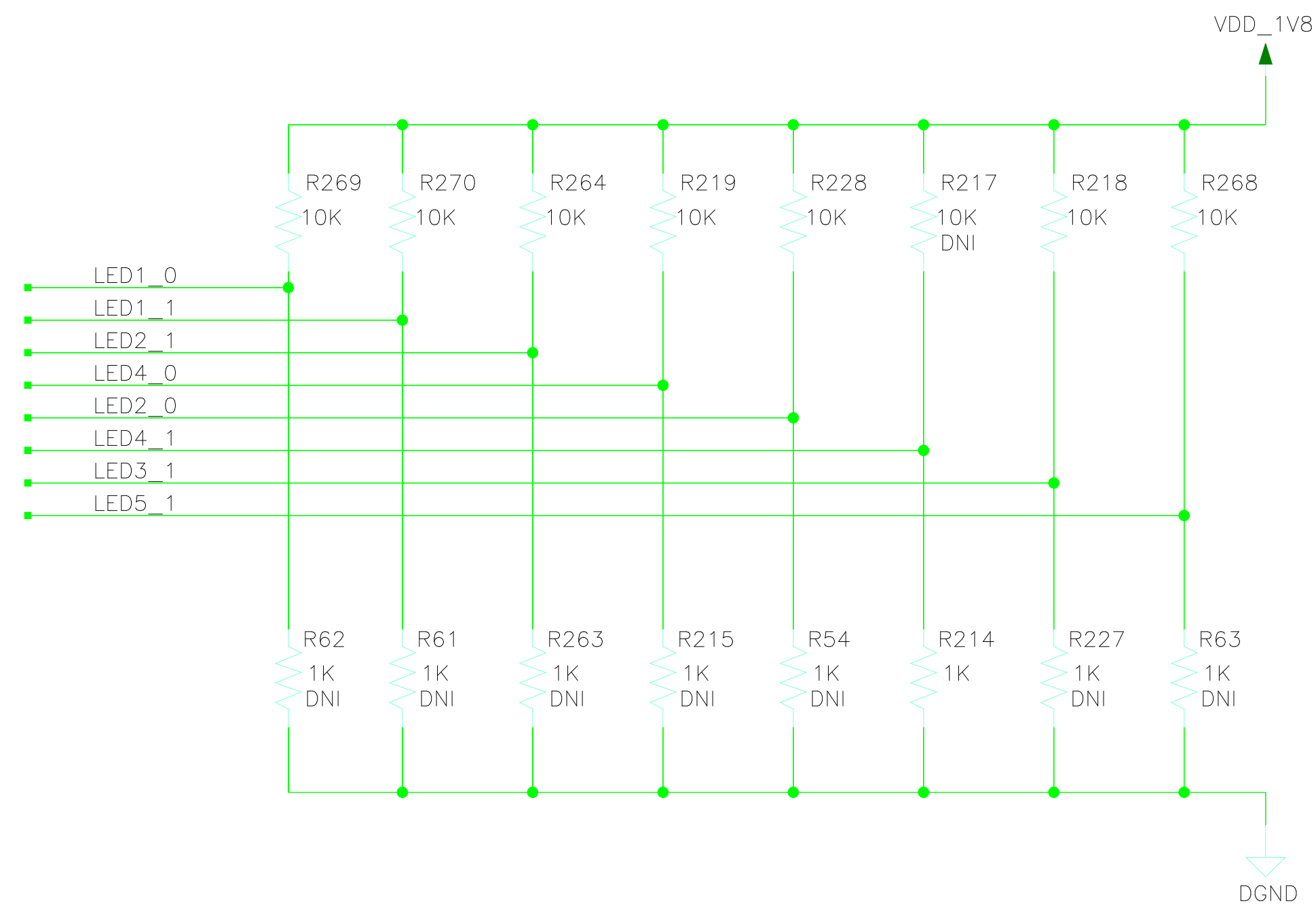
CONFIGURATION STRAP FOR 7-PORT SWITCH
