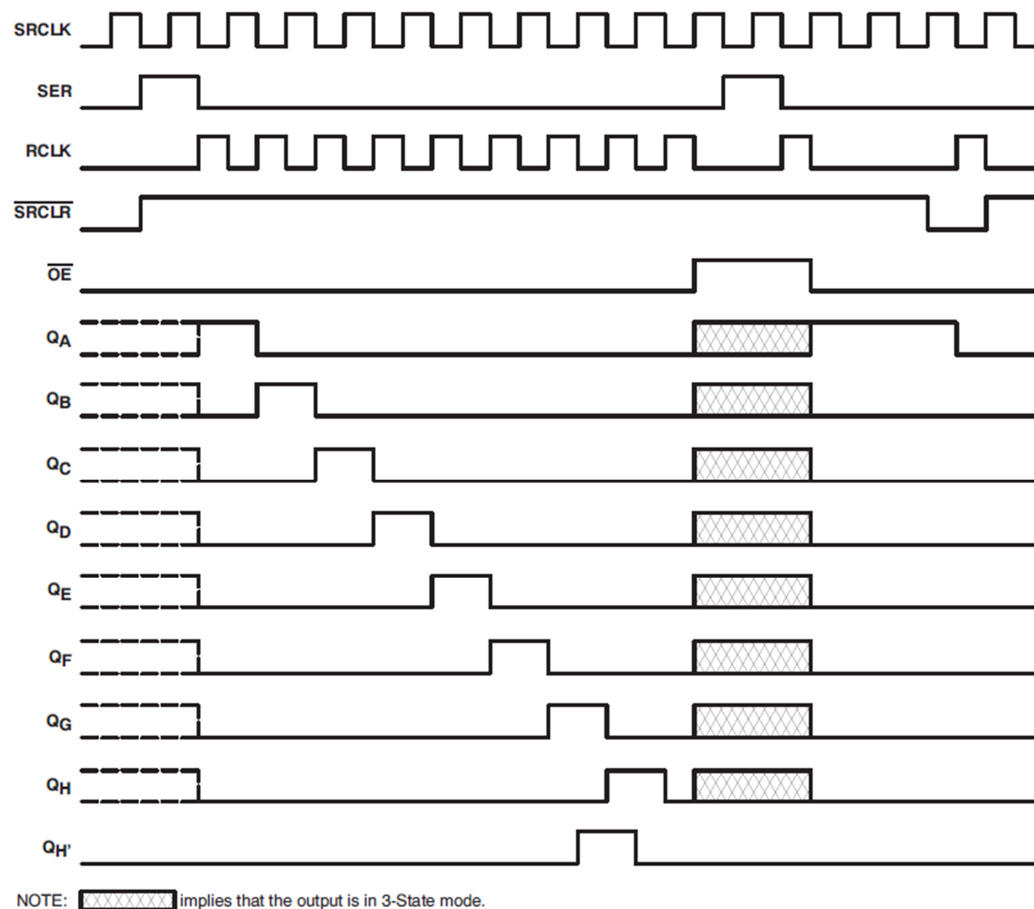
Figure 1. Timing Diagram
